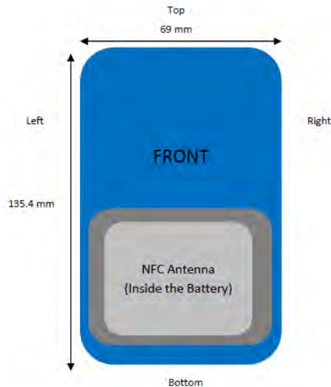
Figure 1-2 DUT Antenna Locations
