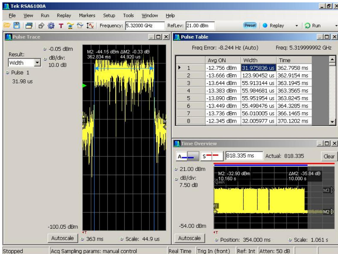
Figure 5-6. Aggregate Time using Pulse Table Capability
