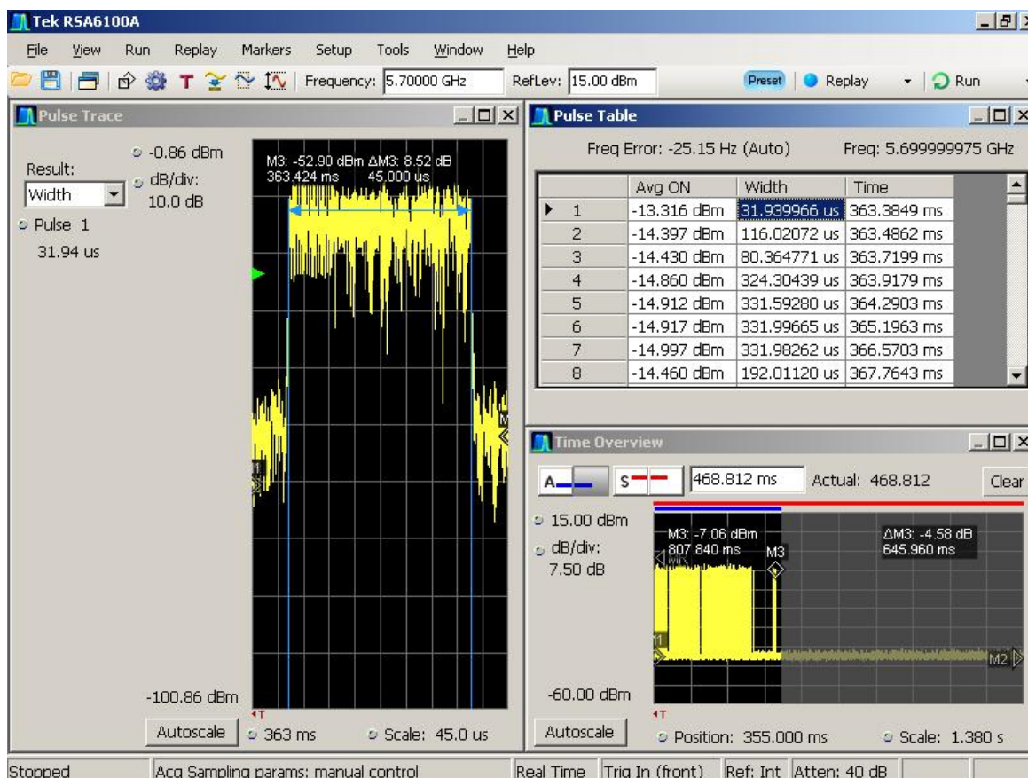
Figure 6-6. Aggregate Time using Pulse Table Capability
