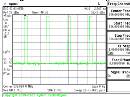
Figure 8-6 GSM850 Signal
