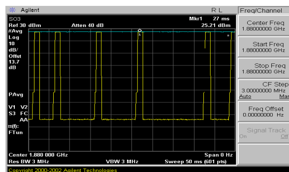
Figure 8-3 Zero-Span Plots
