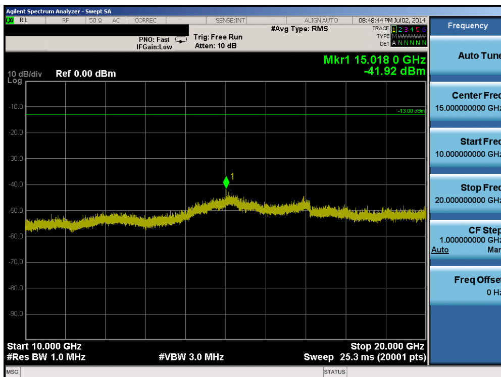
Plot 6-24. Conducted Spurious Plot (Band 25 – 20.0MHz QPSK – RB Size 1, RB Offset 0 – High Channel)
