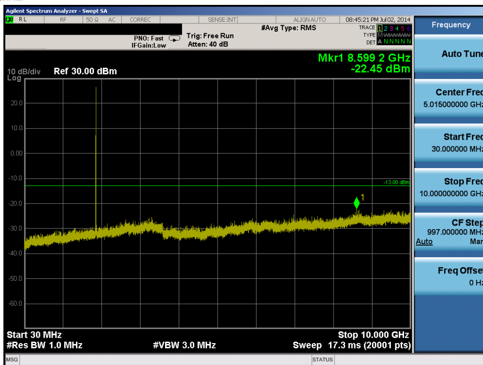
Plot 6-21. Conducted Spurious Plot (Band 25 – 20.0MHz QPSK – RB Size 1, RB Offset 0 – Mid Channel)
