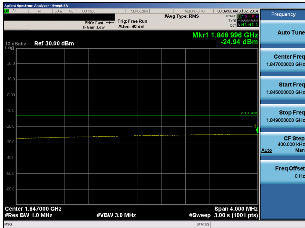
Plot 6-30. Lower Extended Band Edge Plot (Band 25 – 15.0MHz QPSK – RB Size 75)
