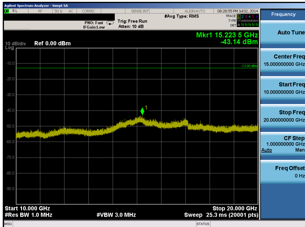
Plot 6-12. Conducted Spurious Plot (Band 25 – 1.4MHz QPSK – RB Size 1, RB Offset 0 – High Channel)
