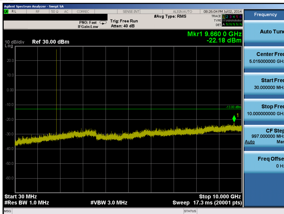
Plot 6-7. Conducted Spurious Plot (Band 25 – 1.4MHz QPSK – RB Size 1, RB Offset 0 – Low Channel)
