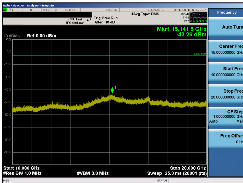
Plot 6-18. Conducted Spurious Plot (Band 25 – 15.0MHz QPSK – RB Size 1, RB Offset 0 – High Channel)
