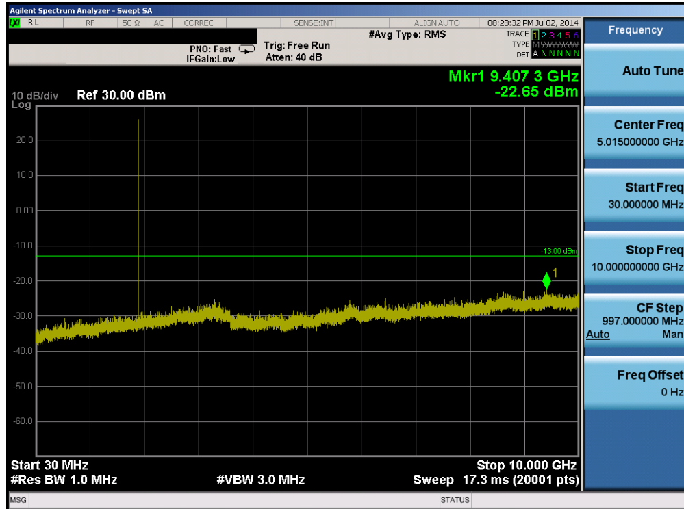
Plot 6-11. Conducted Spurious Plot (Band 25 – 1.4MHz QPSK – RB Size 1, RB Offset 0 – High Channel)
