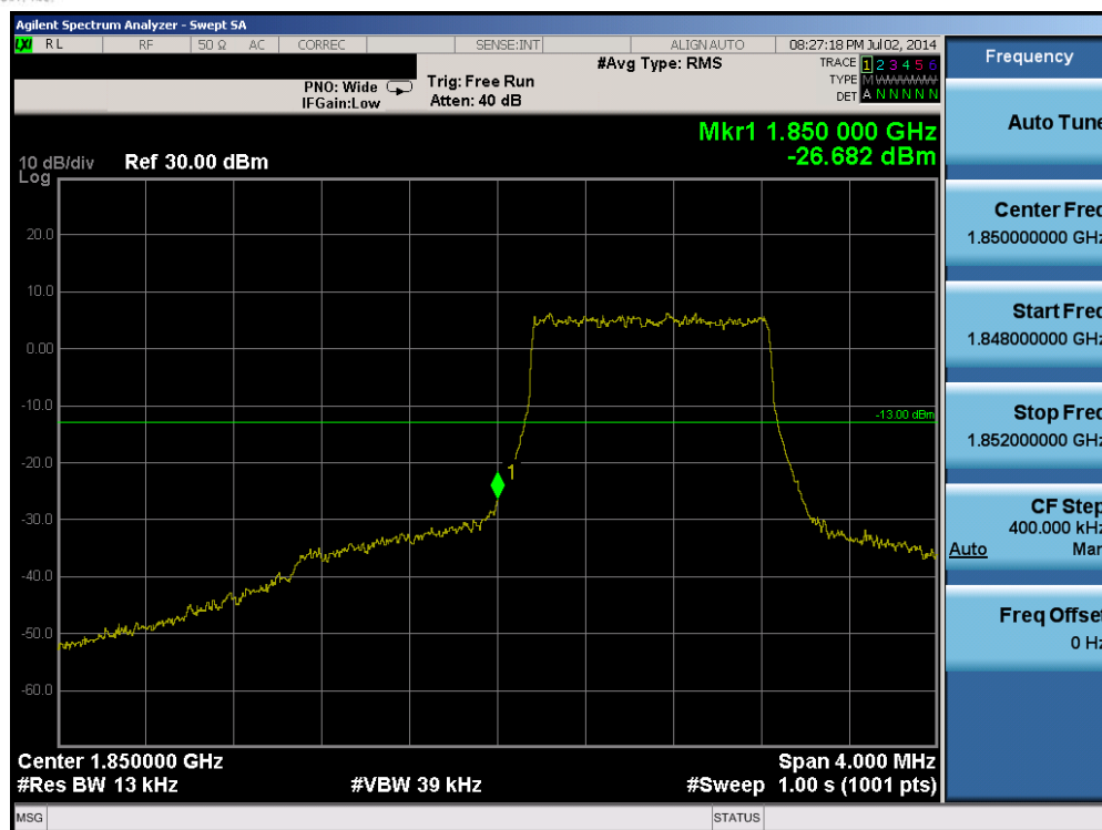
Plot 6-25. Lower Band Edge Plot (Band 25 – 1.4MHz QPSK – RB Size 6)
