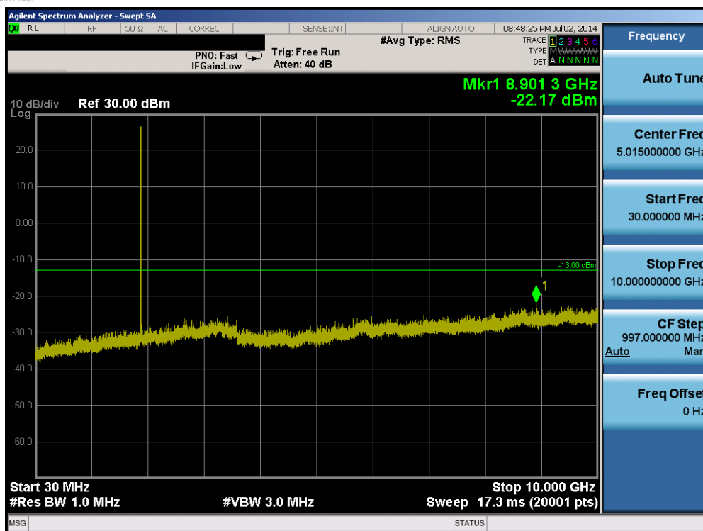
Plot 6-23. Conducted Spurious Plot (Band 25 – 20.0MHz QPSK – RB Size 1, RB Offset 0 – High Channel)
