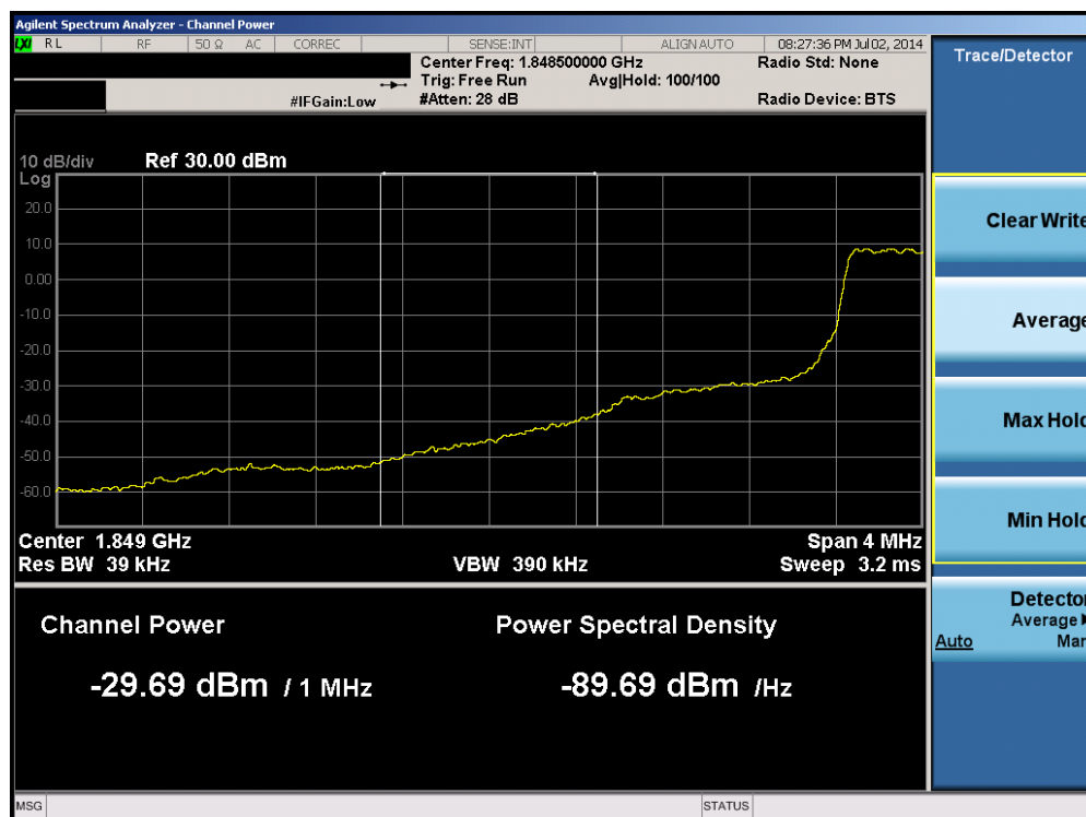
Plot 6-26. Lower Extended Band Edge Plot (Band 25 – 1.4MHz QPSK – RB Size 6)
