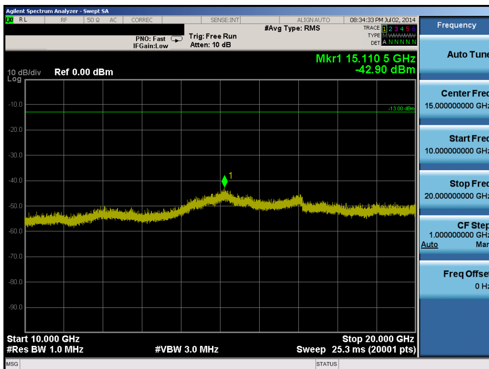
Plot 6-16. Conducted Spurious Plot (Band 25 – 15.0MHz QPSK – RB Size 1, RB Offset 0 – Mid Channel)
