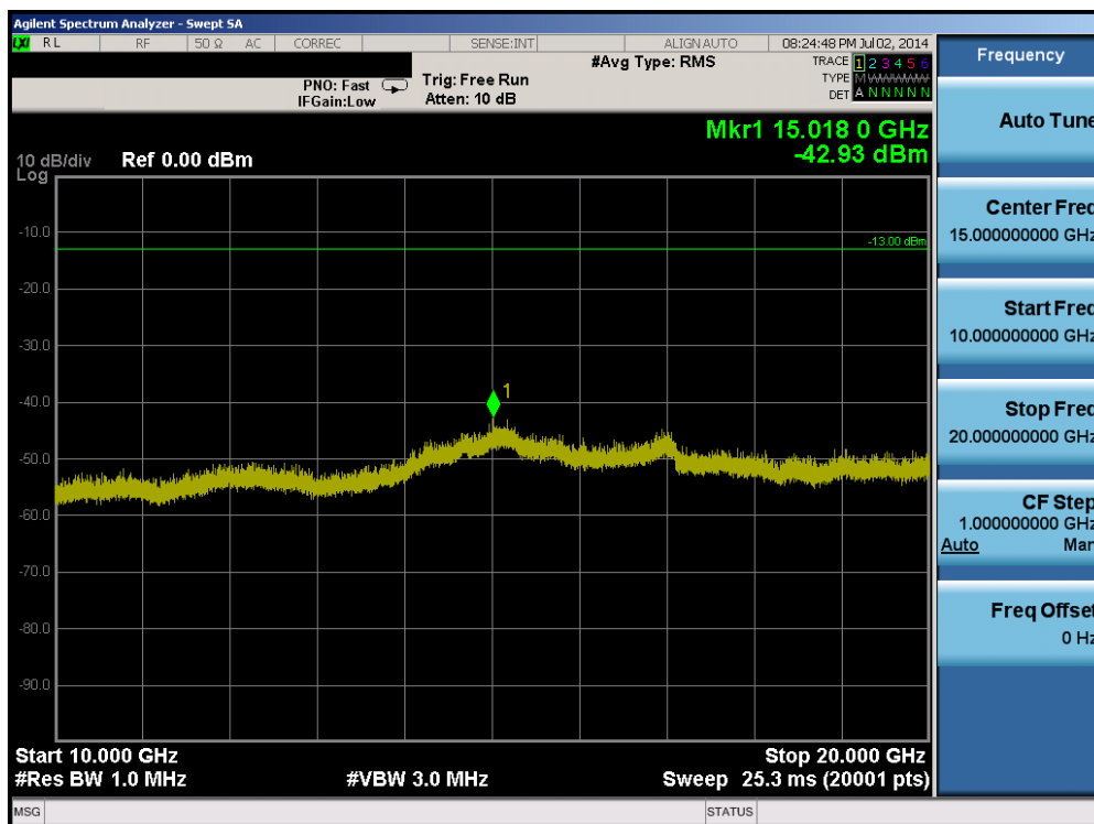
Plot 6-10. Conducted Spurious Plot (Band 25 – 1.4MHz QPSK – RB Size 1, RB Offset 0 – Mid Channel)
