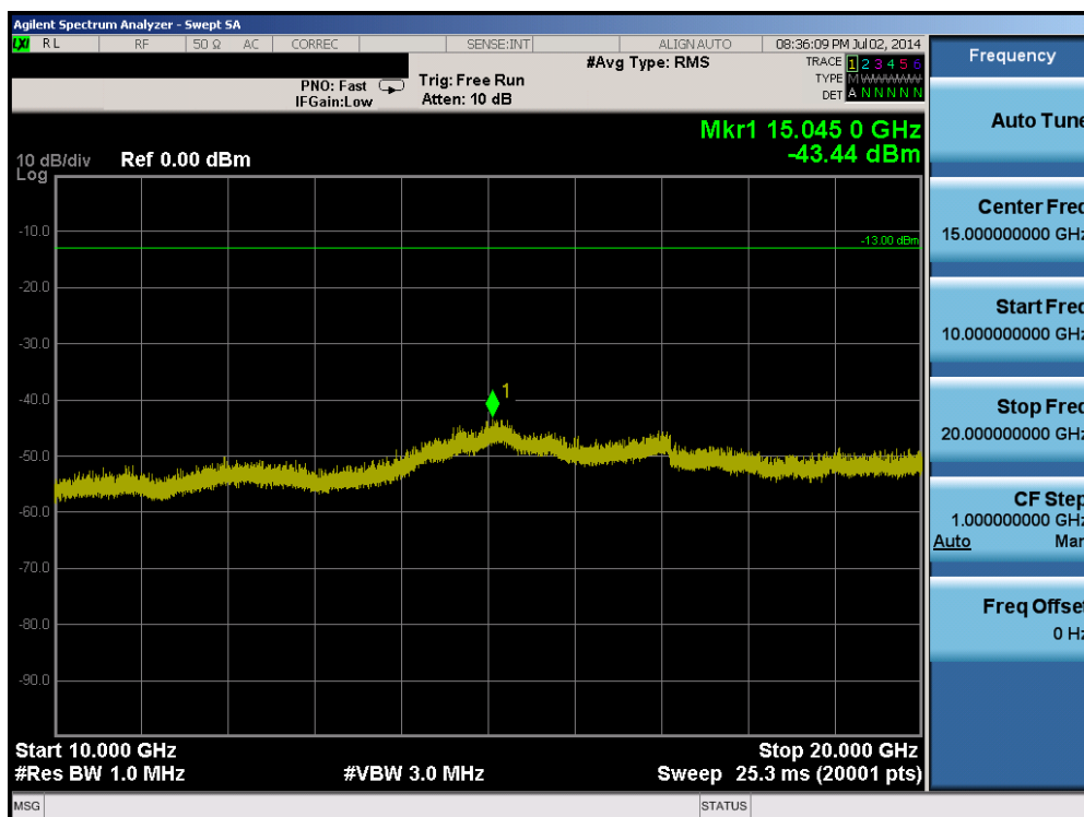
Plot 6-14. Conducted Spurious Plot (Band 25 – 15.0MHz QPSK – RB Size 1, RB Offset 0 – Low Channel)
