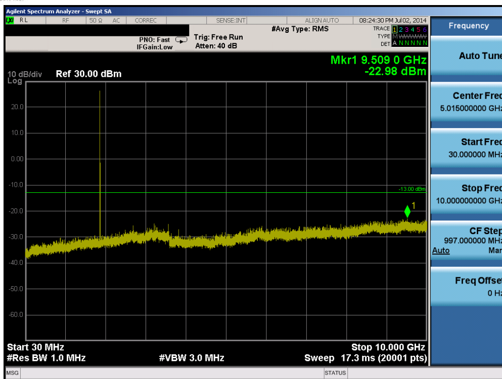
Plot 6-9. Conducted Spurious Plot (Band 25 – 1.4MHz QPSK – RB Size 1, RB Offset 0 – Mid Channel)
