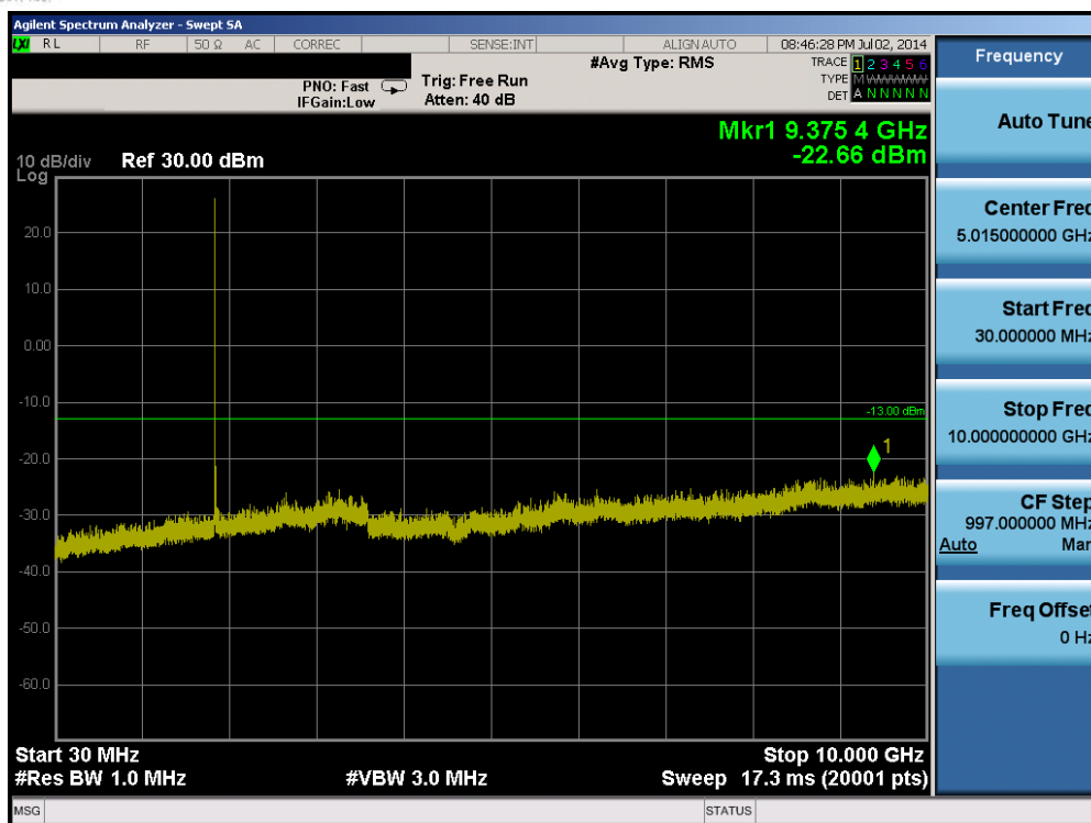
Plot 6-19. Conducted Spurious Plot (Band 25 – 20.0MHz QPSK – RB Size 1, RB Offset 0– Low Channel)
