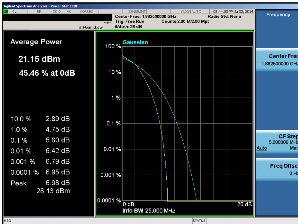
Plot 6-42. PAR Plot (Band 25 – 20.0MHz 16-QAM – RB Size 100)
