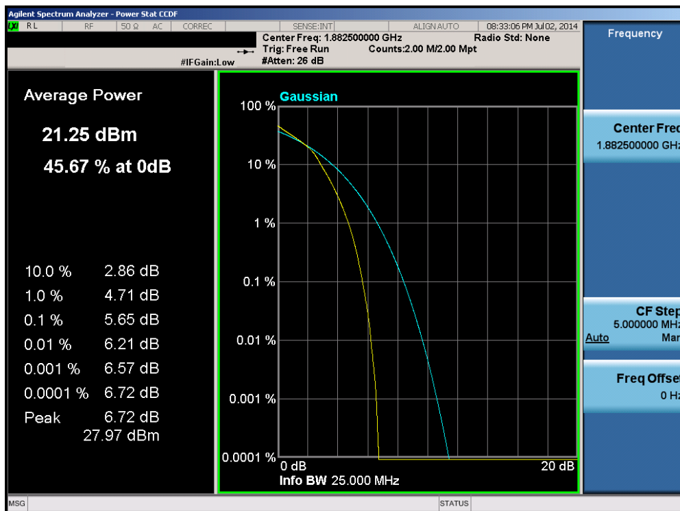
Plot 6-40. PAR Plot (Band 25 – 15.0MHz 16-QAM – RB Size 75)
