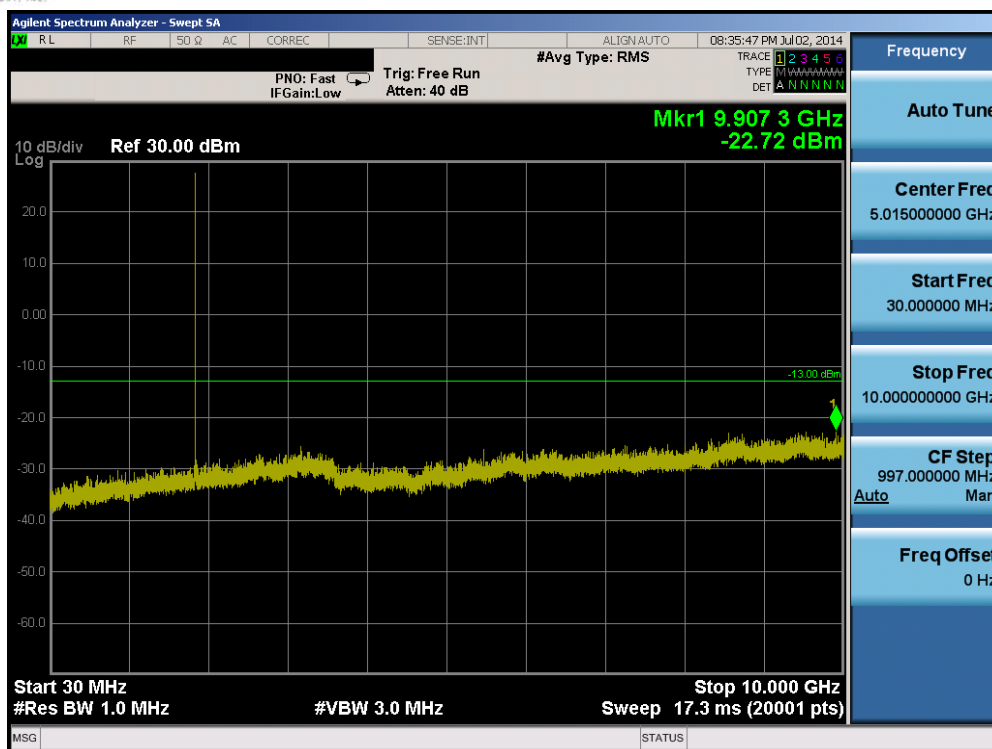
Plot 6-13. Conducted Spurious Plot (Band 25 – 15.0MHz QPSK – RB Size 1, RB Offset 0 – Low Channel)
