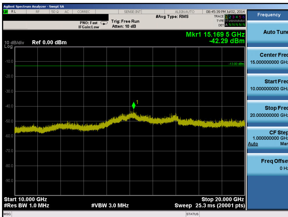
Plot 6-22. Conducted Spurious Plot (Band 25 – 20.0MHz QPSK – RB Size 1, RB Offset 0 – Mid Channel)
