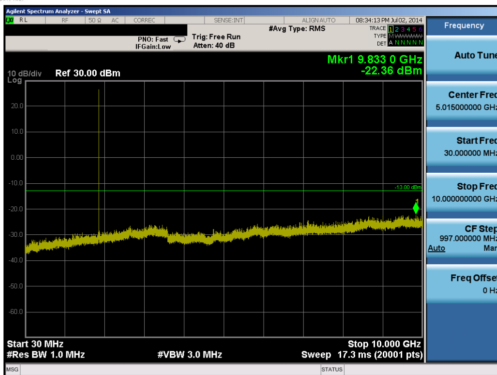
Plot 6-15. Conducted Spurious Plot (Band 25 – 15.0MHz QPSK – RB Size 1, RB Offset 0 – Mid Channel)
