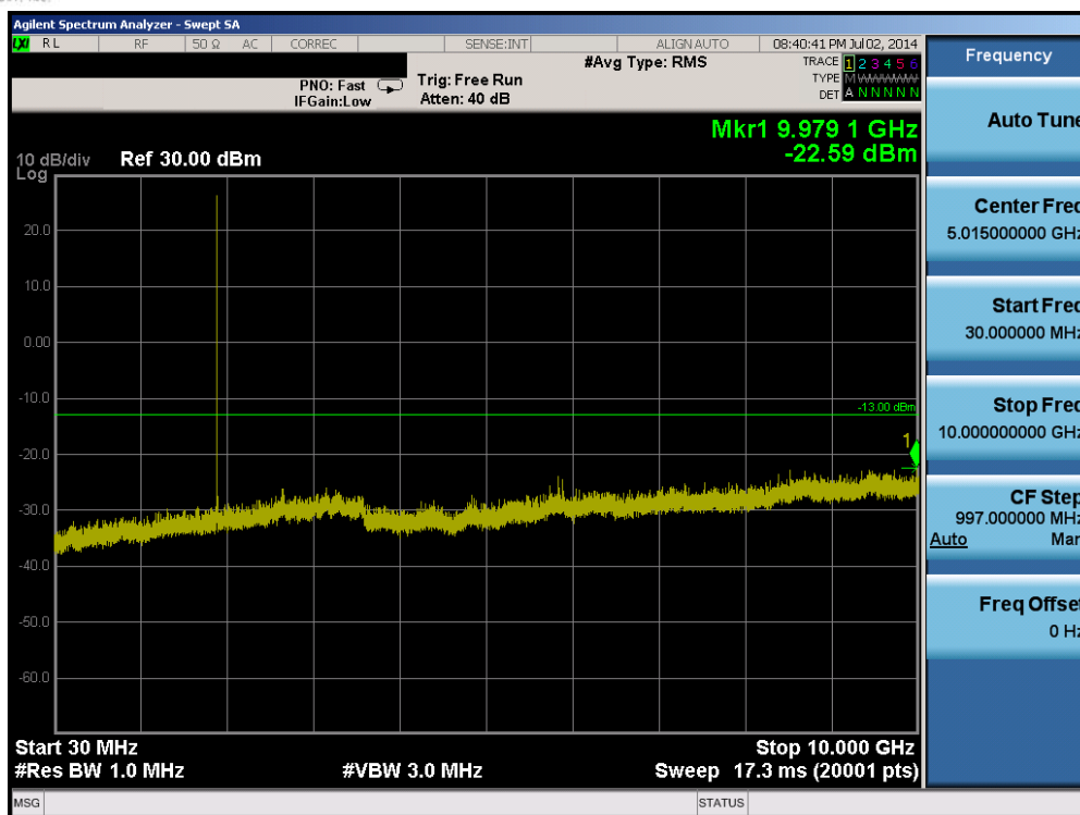
Plot 6-17. Conducted Spurious Plot (Band 25 – 15.0MHz QPSK – RB Size 1, RB Offset 0 – High Channel)
