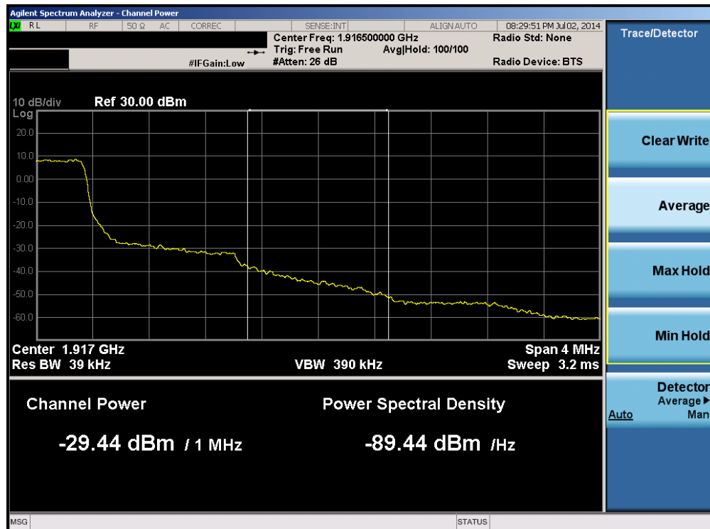
Plot 6-28. Upper Extended Band Edge Plot (Band 25 – 1.4MHz QPSK – RB Size 6)
