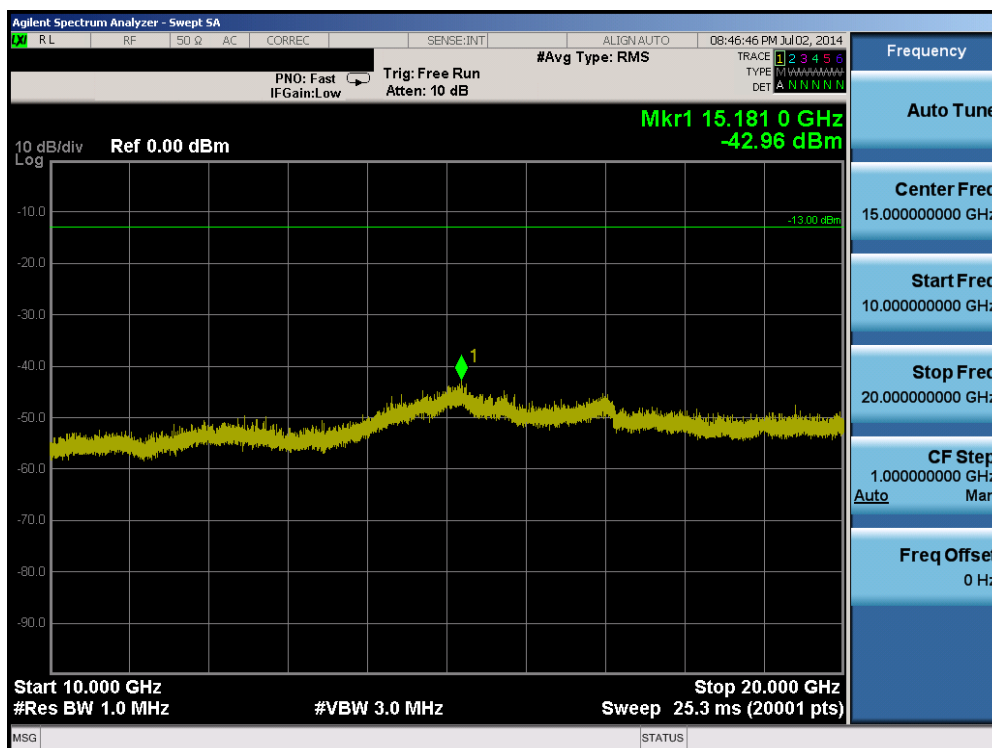
Plot 6-20. Conducted Spurious Plot (Band 25 – 20.0MHz QPSK – RB Size 1, RB Offset 0 – Low Channel)
