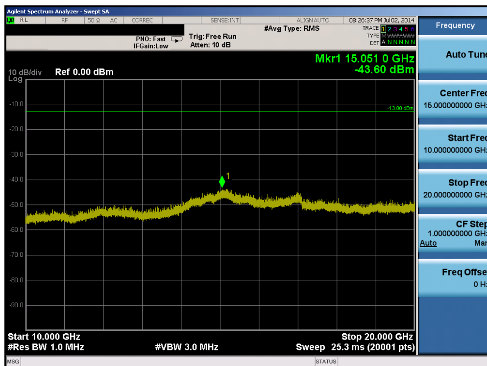
Plot 6-8. Conducted Spurious Plot (Band 25 – 1.4MHz QPSK – RB Size 1, RB Offset 0 – Low Channel)
