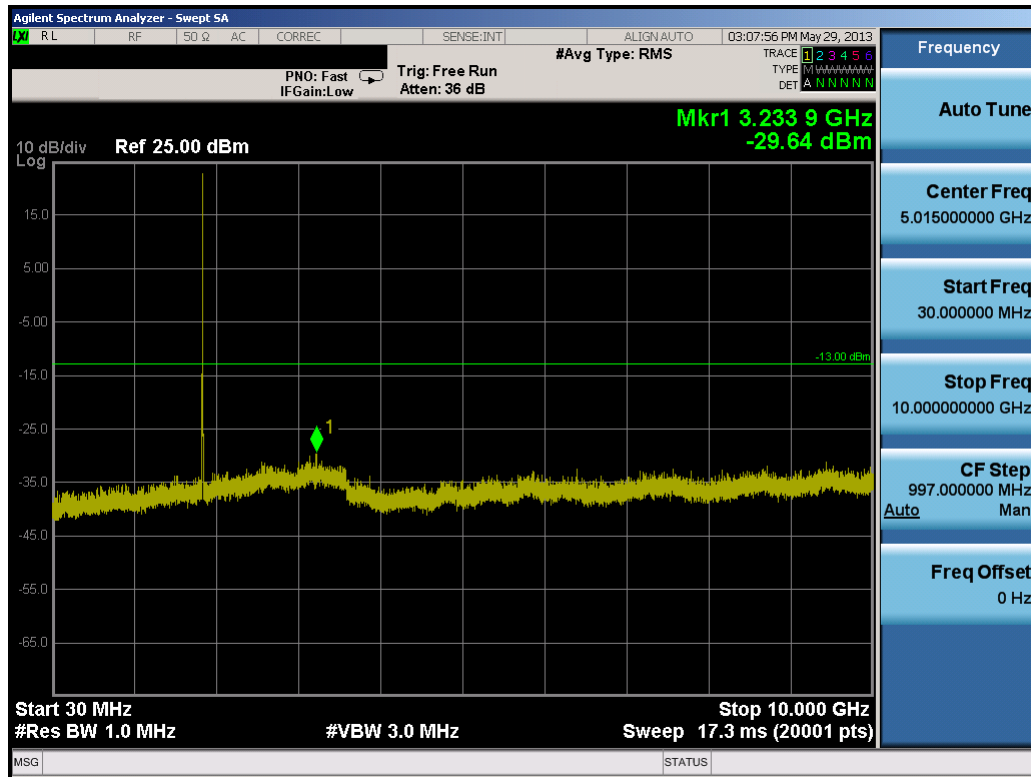
Plot 7-49. Conducted Spurious Plot (PCS WCDMA Mode – Ch. 9262)
