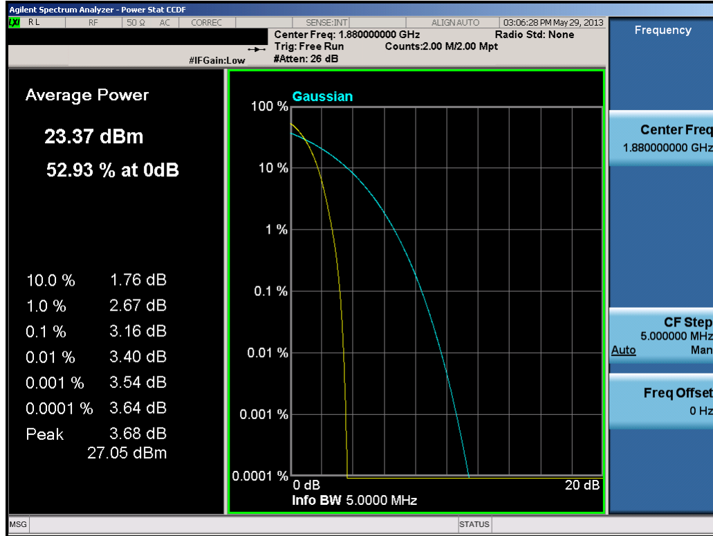
Plot 7-56. Peak-Average Ratio Plot (PCS WCDMA Mode – Ch. 9400)
