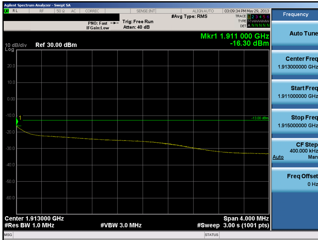
Plot 7-60. 4MHz Span Plot (PCS WCDMA Mode – Ch. 9538)
