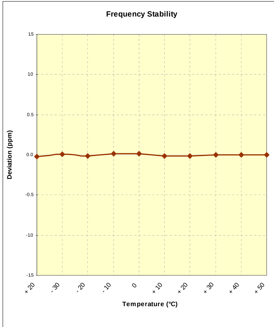
Figure 6-4. Frequency Stability Graph (PCS CDMA Mode – Ch. 600)
