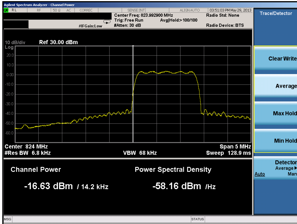
Plot 7-28. Band Edge Plot (Cellular CDMA Mode – Ch. 1013)
