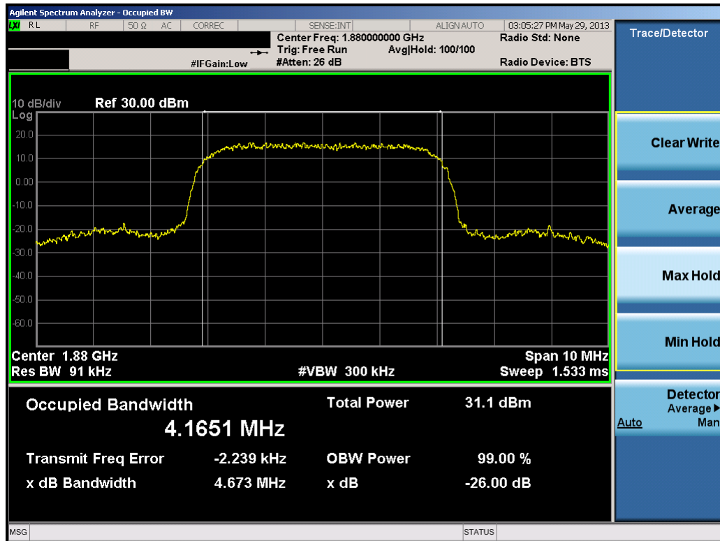
Plot 7-55. Occupied Bandwidth Plot (PCS WCDMA Mode – Ch. 9400)
