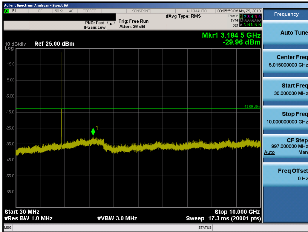
Plot 7-53. Conducted Spurious Plot (PCS WCDMA Mode – Ch. 9400)
