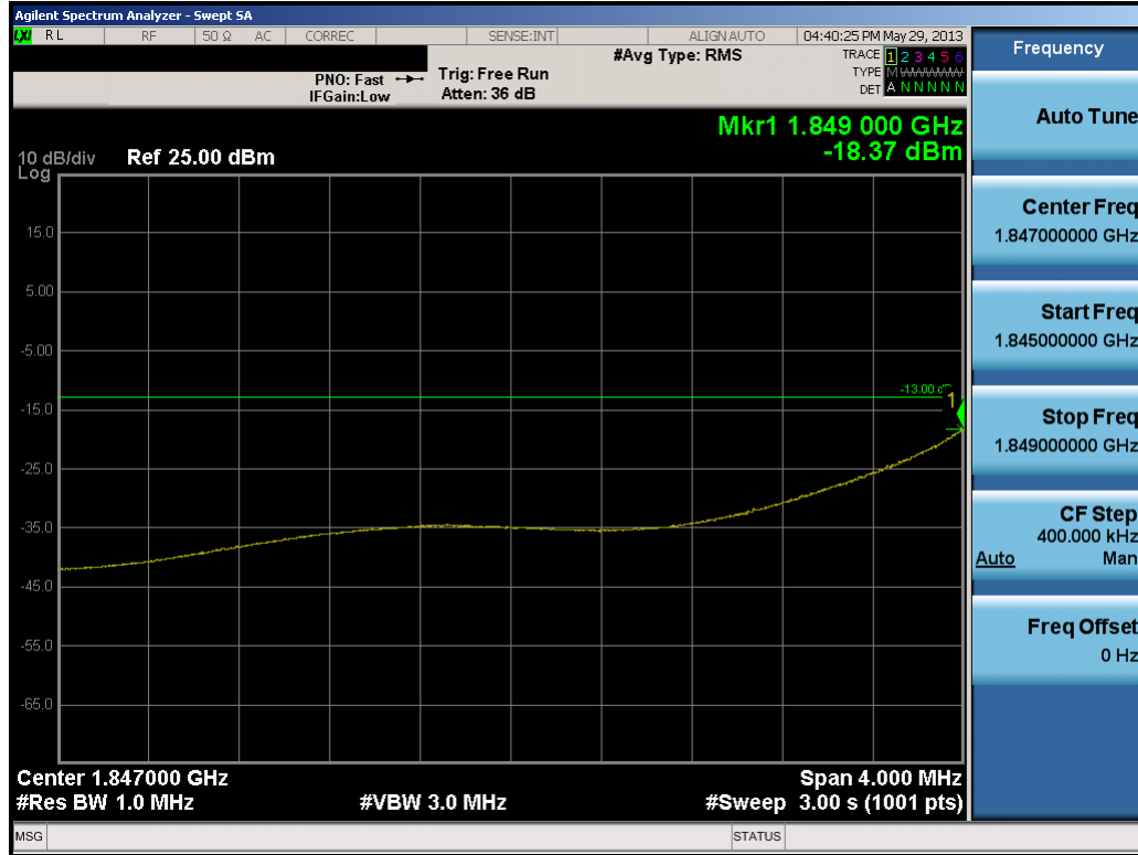
Plot 7-40. 4MHz Span Plot (PCS CDMA Mode – Ch. 25)
