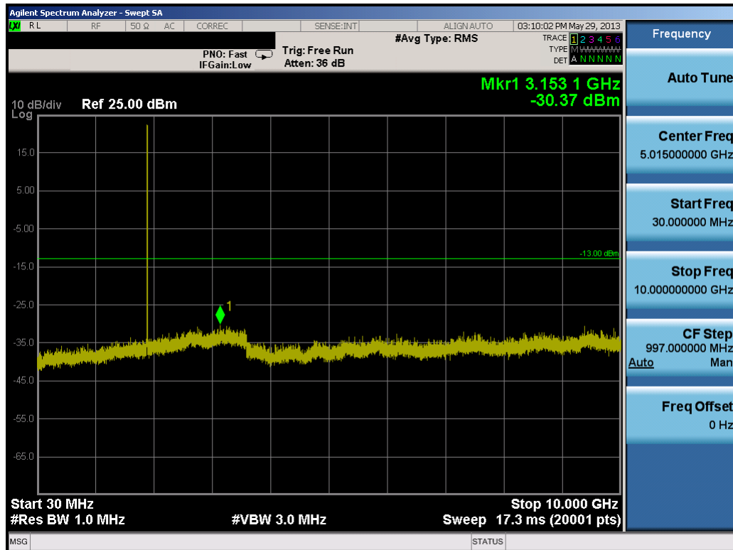
Plot 7-57. Conducted Spurious Plot (PCS WCDMA Mode – Ch. 9538)
