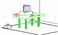
Figure 3-3. Wooden Table & Bonded LISNs
