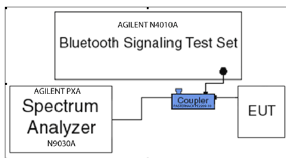
Figure 6-1. Test Instrument & Measurement Setup
