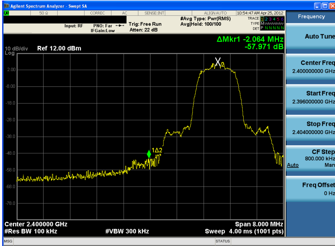
Plot 6-10. Band Edge Plot (Bluetooth with Hopping Disabled, 3Mbps – Ch. 0)
