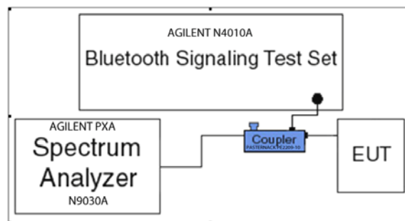
Figure 6-2. Test Instrument & Measurement Setup
