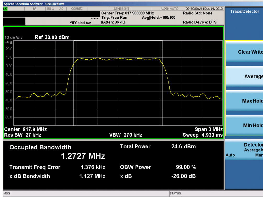
Plot 7-13. Occupied Bandwidth Plot (Ch. 476)
