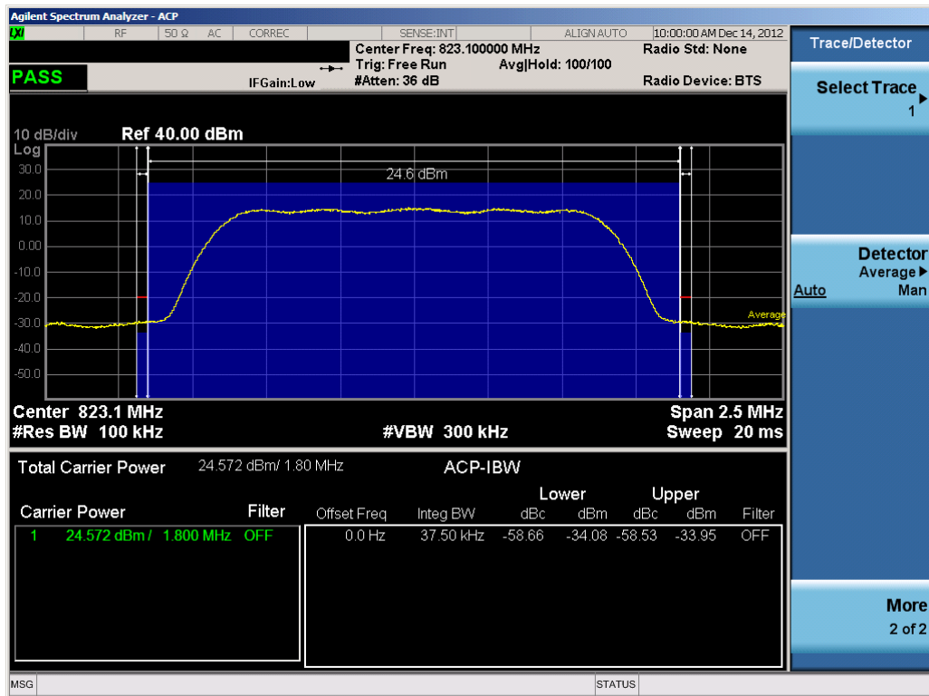
Plot 7-10. Channel Edge Plot (Ch. 684)
