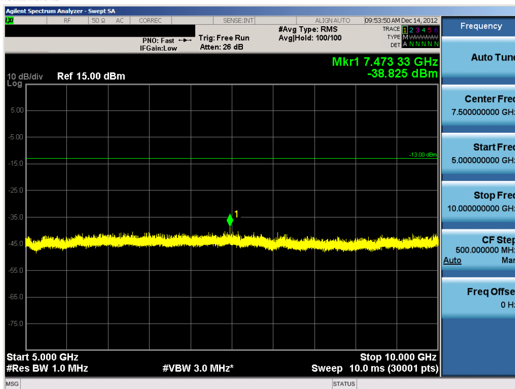
Plot 7-3. Conducted Spurious Plot (Ch. 476)
