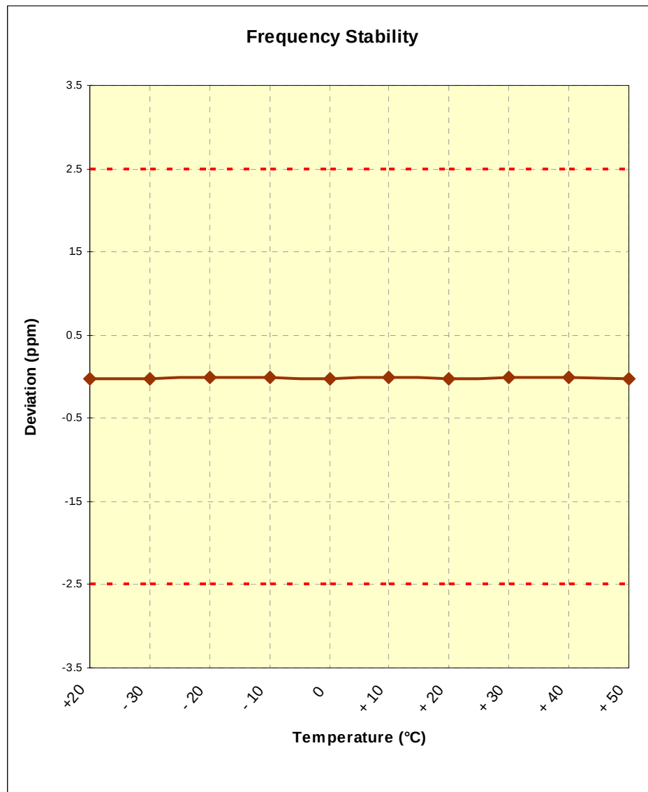
Figure 6-1. Frequency Stability Graph (Ch. 684)
