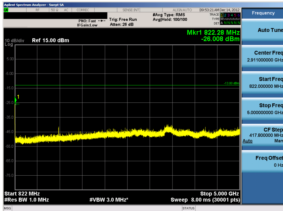
Plot 7-2. Conducted Spurious Plot (Ch. 476)
