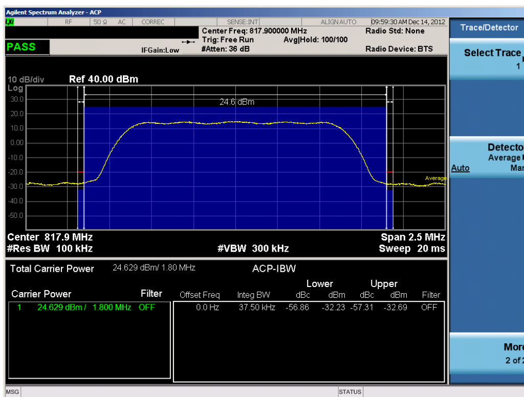
Plot 7-4. Channel Edge Plot (Ch. 476)
