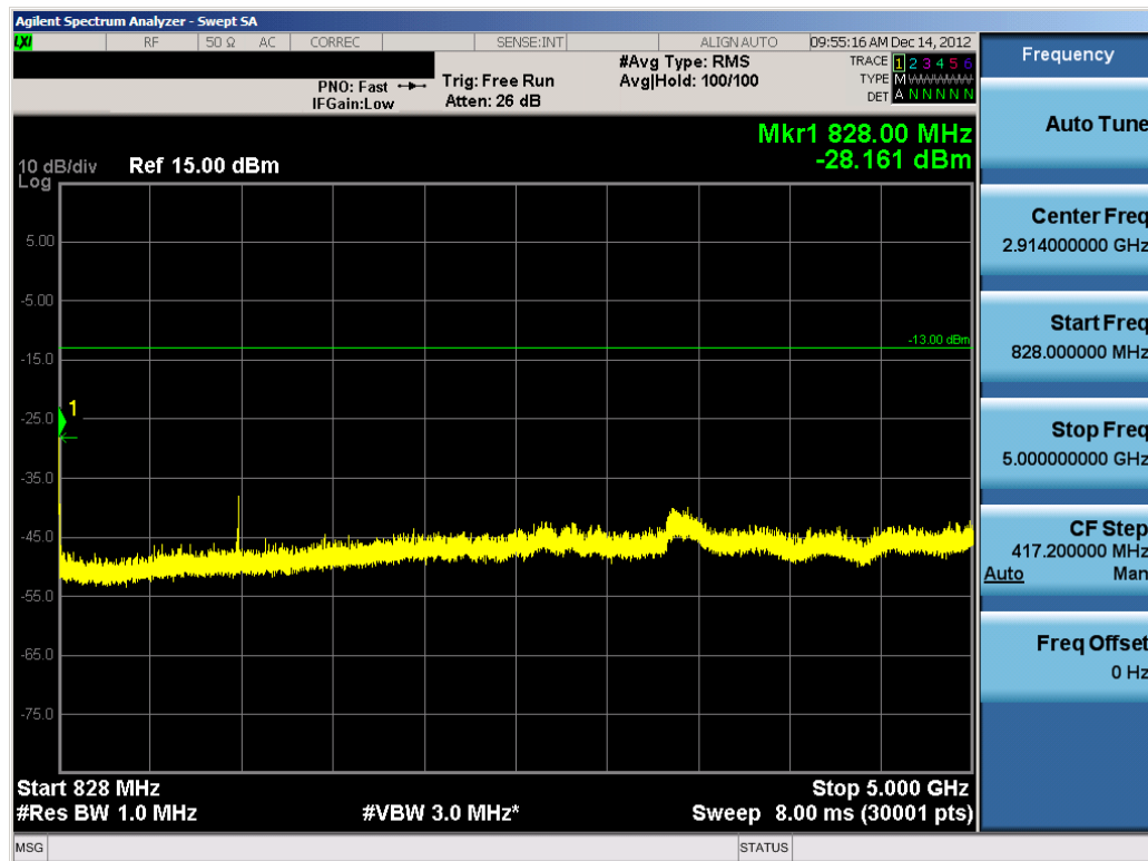
Plot 7-8. Conducted Spurious Plot (Ch. 684)
