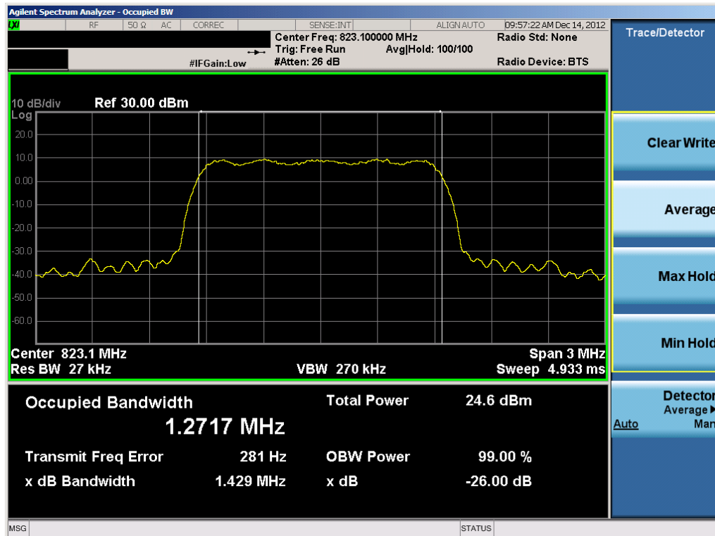
Plot 7-14. Occupied Bandwidth Plot (Ch. 684)
