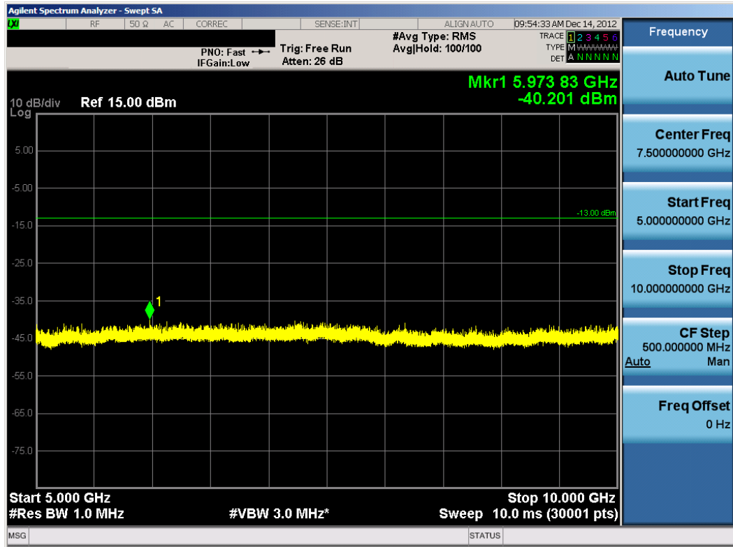
Plot 7-9. Conducted Spurious Plot (Ch. 684)
