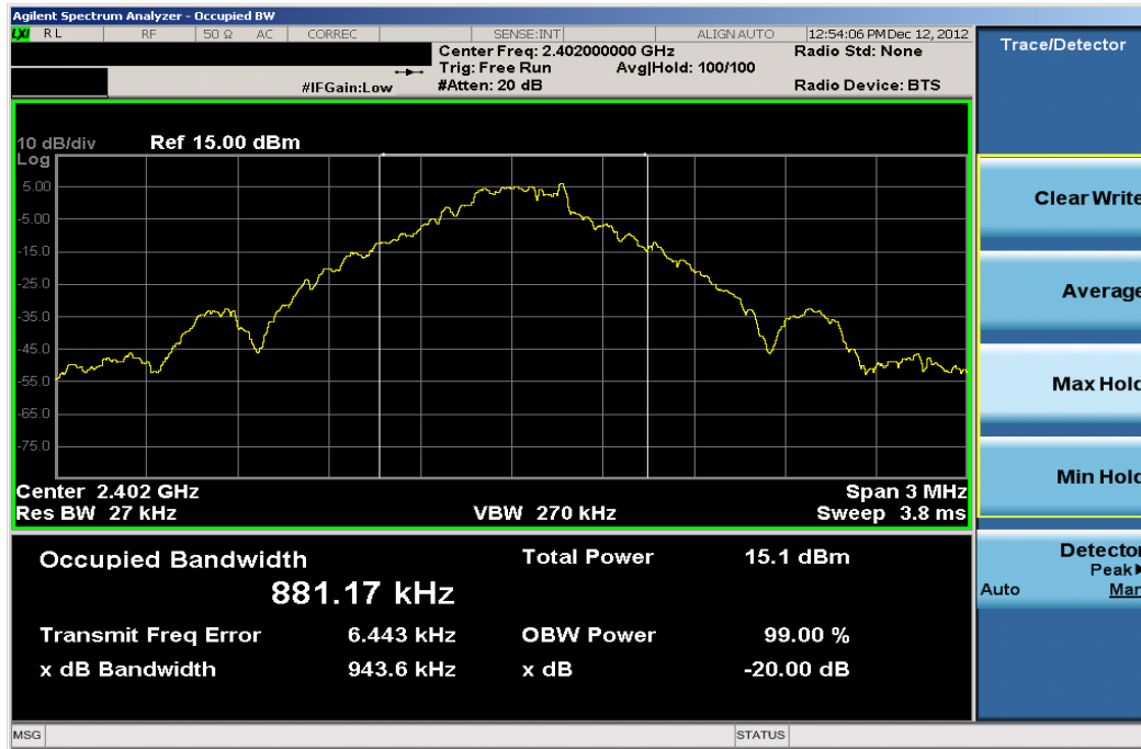
Plot 6-1. 20dB Bandwidth Plot (Bluetooth, 1Mbps – Ch. 0)
