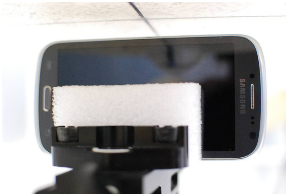
SAR Test Setup Photo 10 – Left Edge
