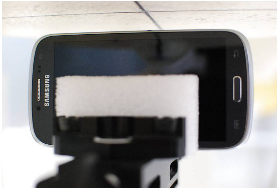
SAR Test Setup Photo 9 – Right Edge
