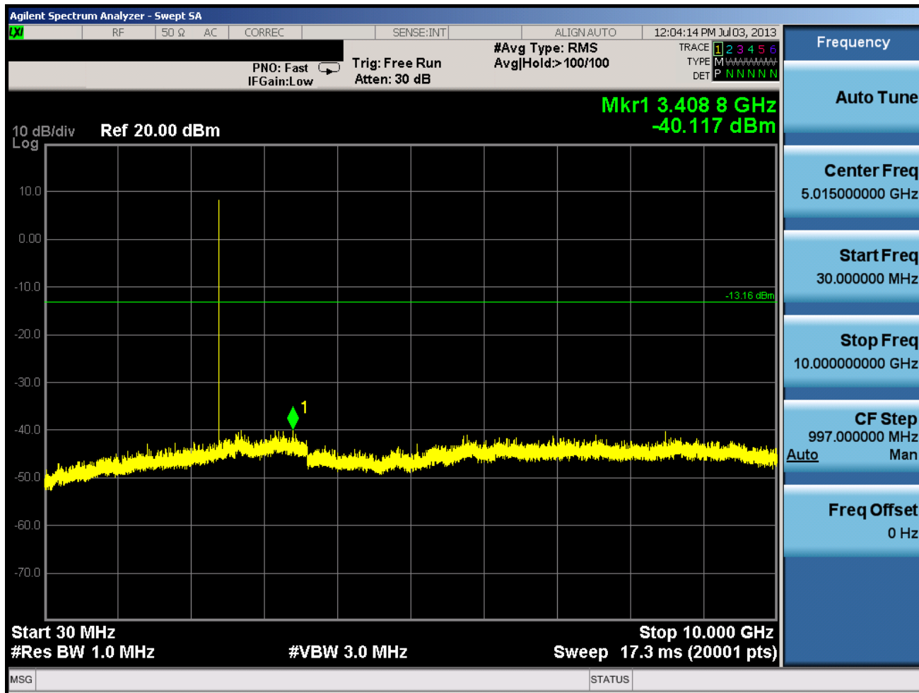
Plot 6-36. Conducted Spurious Plot (Bluetooth, 1Mbps – Ch. 0)
