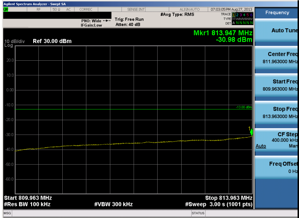
Plot 7-49. Extended Band Edge Plot (10MHz QPSK - RB Size 50 - High Channel)
