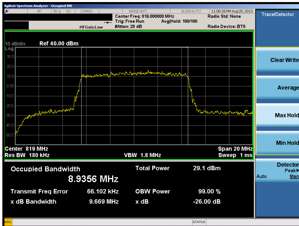
Plot 7-48. Occupied Bandwidth Plot (10MHz QPSK – RB Size 50 – High Channel)
