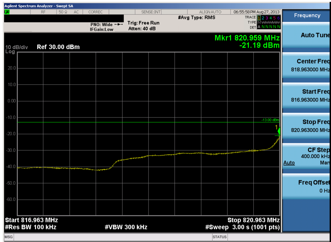
Plot 7-34. Extended Band Edge Plot (3MHz QPSK - RB Size 15 - High Channel)
