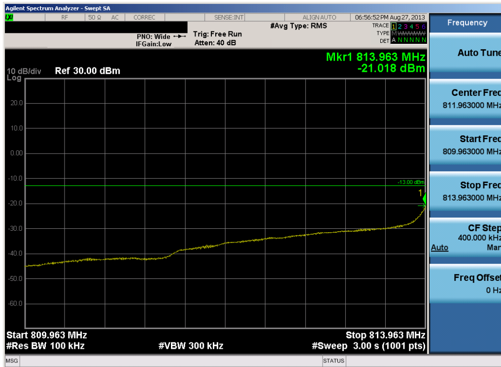
Plot 7-28. Extended Band Edge Plot (3MHz QPSK – RB Size 15– Low Channel)
