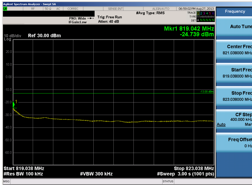
Plot 7-39. Extended Band Edge Plot (5MHz QPSK – RB Size 25– Low Channel)
