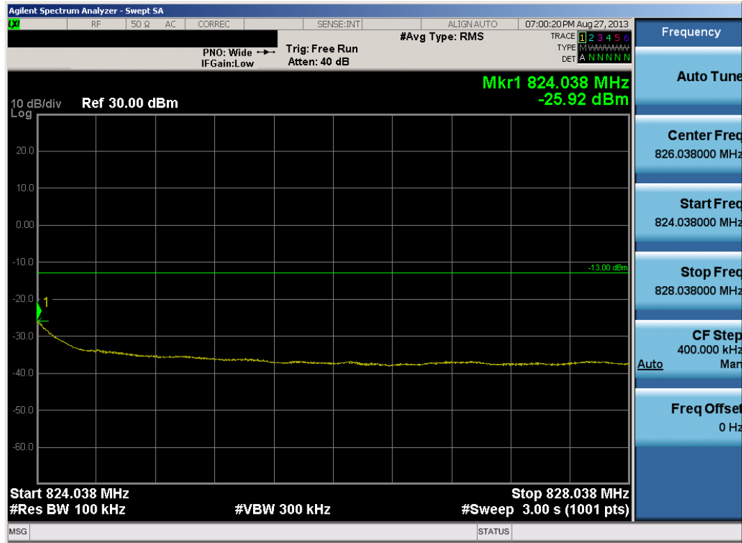
Plot 7-43. Extended Band Edge Plot (5MHz QPSK – RB Size 25 – High Channel)
