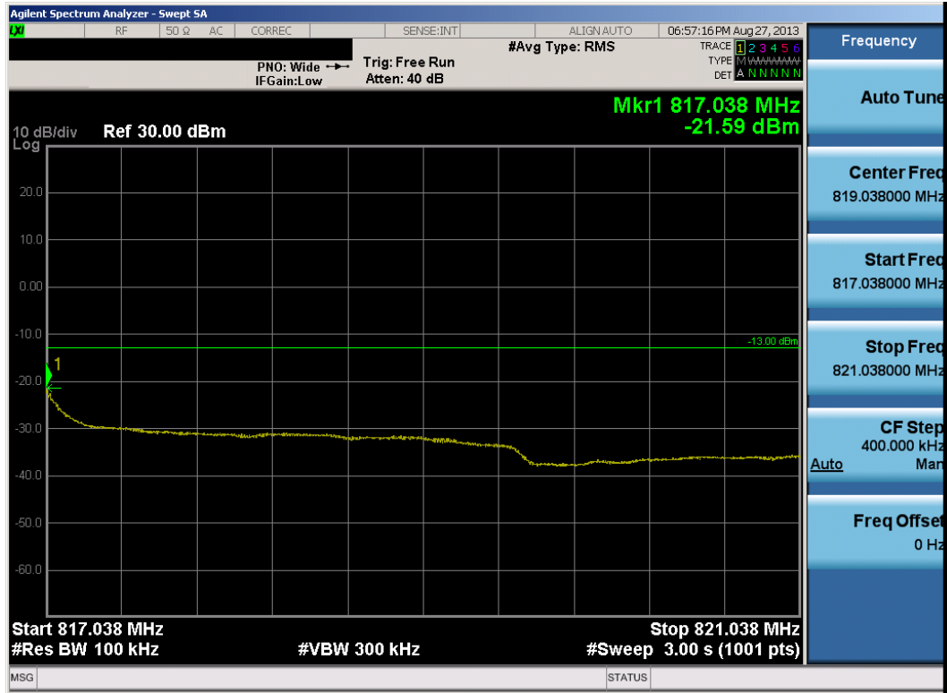
Plot 7-29. Extended Band Edge Plot (3MHz QPSK – RB Size 15– Low Channel)
