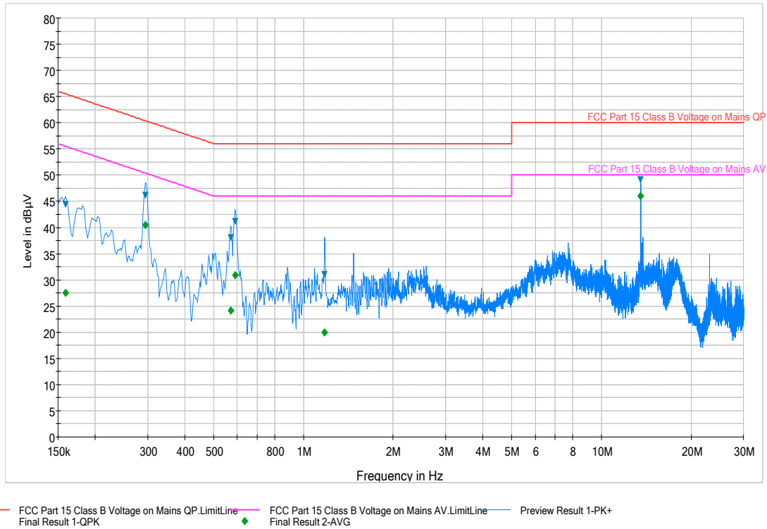
Plot 8-2. Line-Conducted Test Plot (N)
