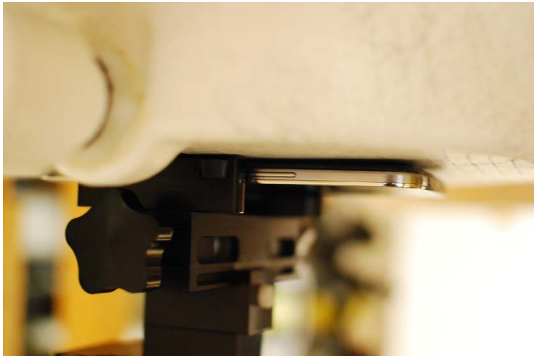
SAR Test Setup Photo 10: Back at 0.0 cm
