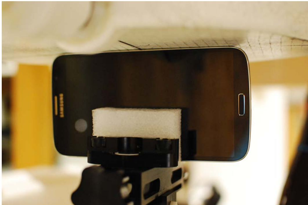
SAR Test Setup Photo 12: Right at 0.0 cm
