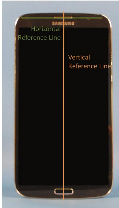
SAR Test Setup Photo 9: Vertical and Horizontal Reference Lines
