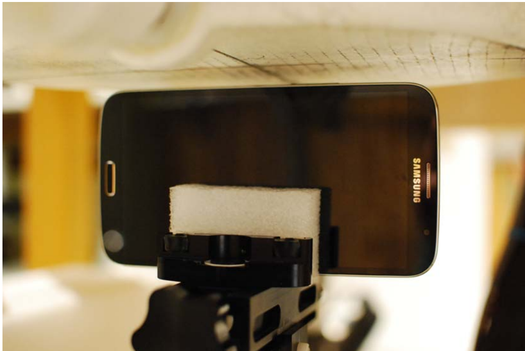
SAR Test Setup Photo 8: Left at 1.0 cm
