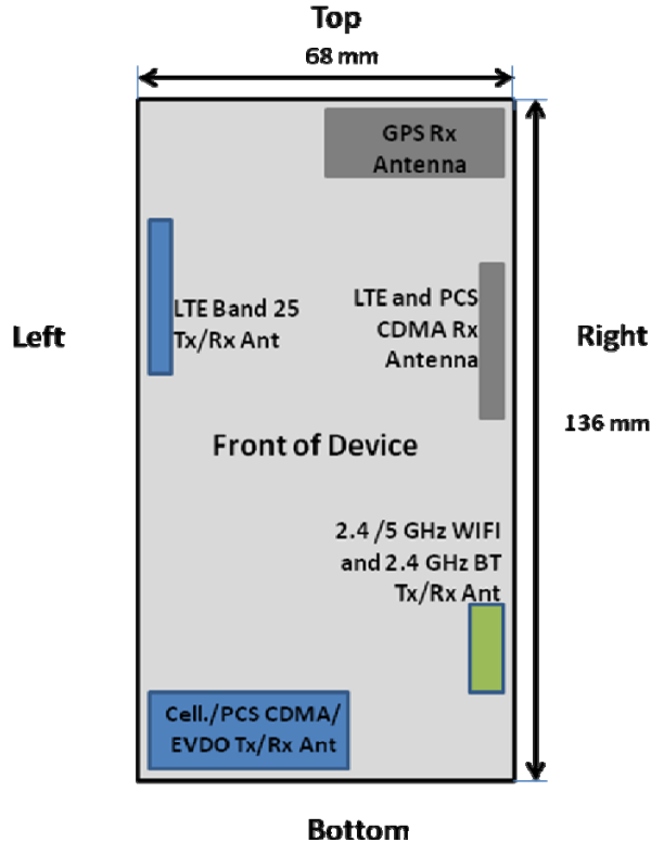
Figure 1-2 EUT Antenna Locations
