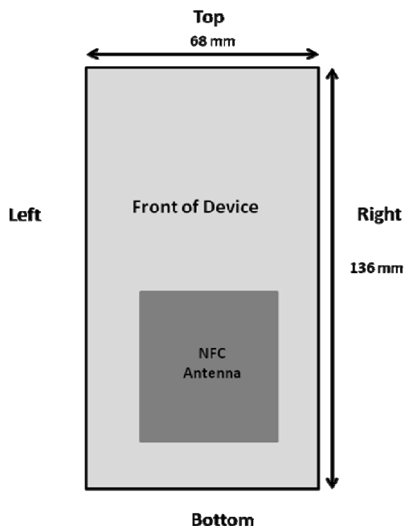
Figure 1-1 NFC Antenna Location on the Battery
