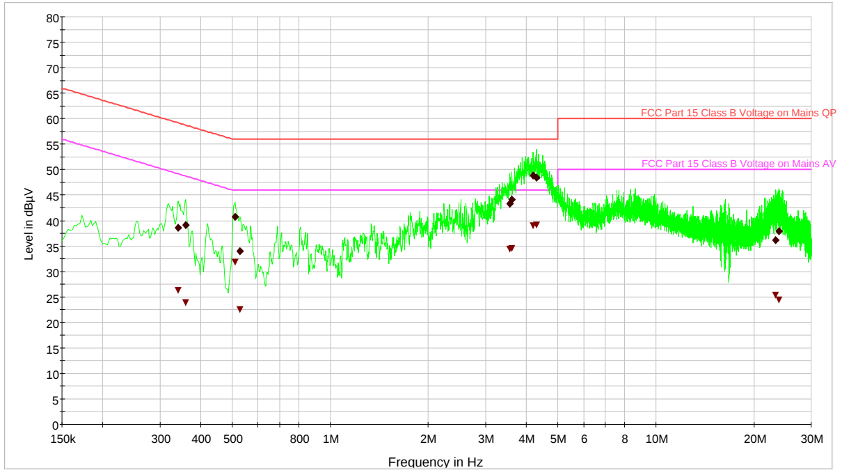
Plot 6-59. Line Conducted Plot with 802.11a (LN)
