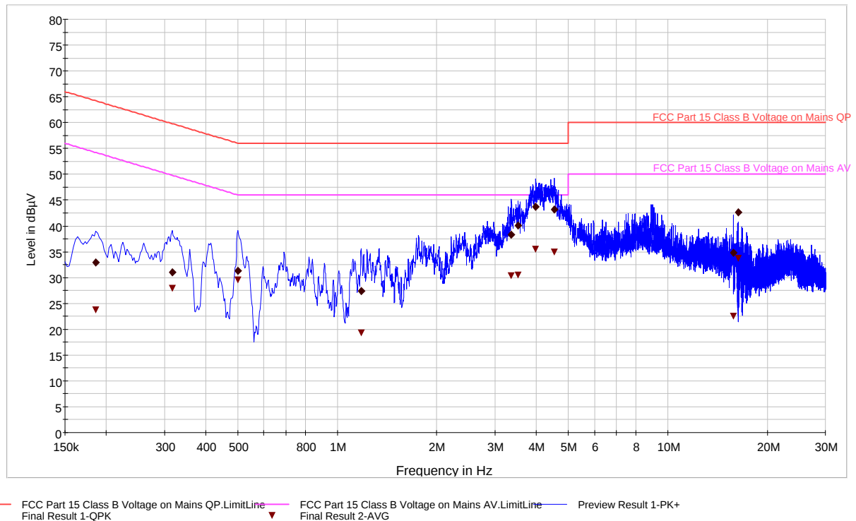
Plot 6-53. Line Conducted Plot with 802.11b
