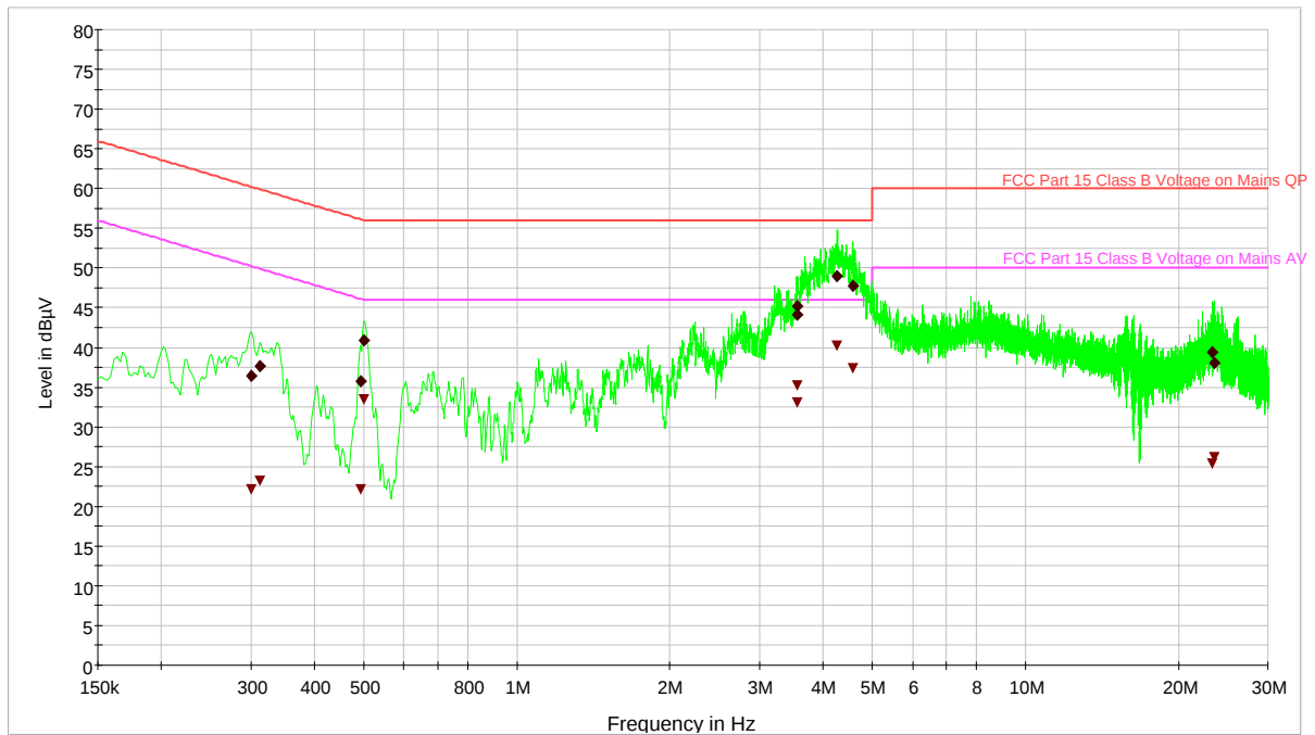
Plot 6-57. Line Conducted Plot with 802.11b
