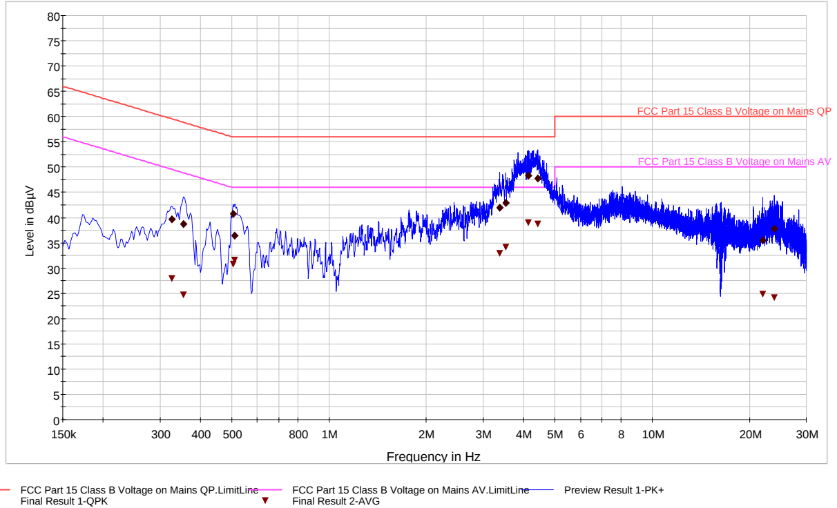
Plot 6-58. Line Conducted Plot with 802.11a (L1)
