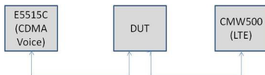
Figure 10-1 SVLTE Conducted Test Setup Diagram
