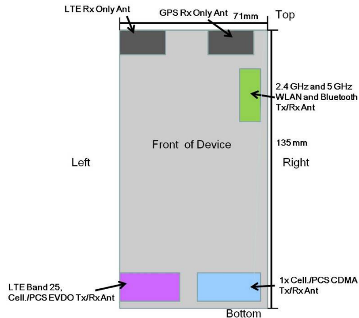
Figure 1-1 DUT Antenna Locations
