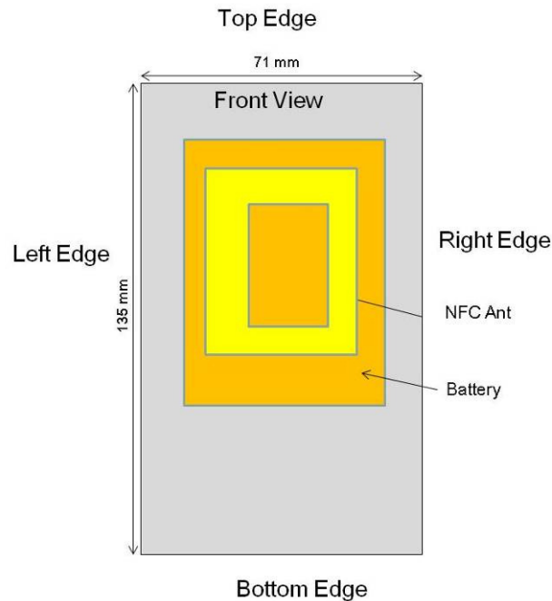
Figure 1-2 DUT Antenna Locations
