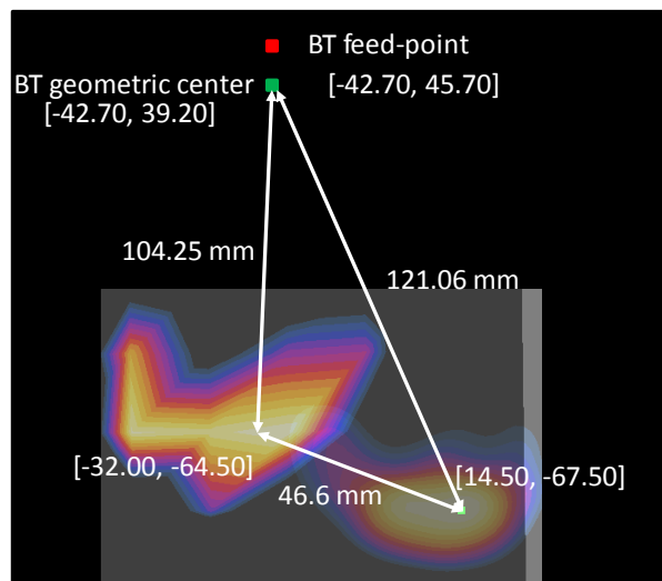
Figure 13-1 Peak SAR Locations of 2.4 GHz Bluetooth, CDMA 1900, and LTE B25
