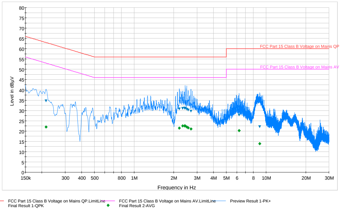
Plot 6-62. Line Conducted Plot with 802.11b (L1)
