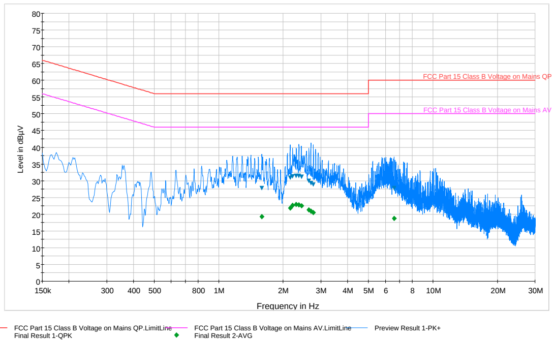
Plot 6-64. Line Conducted Plot with 802.11a (L1)
