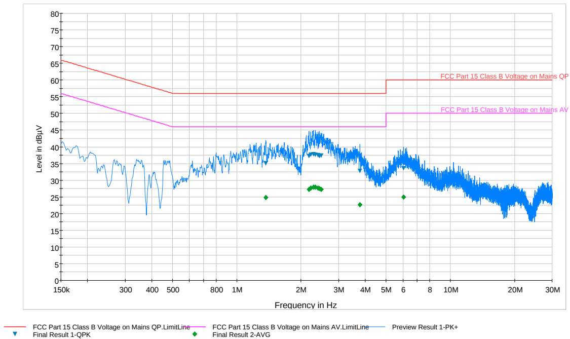
Plot 6-63. Line Conducted Data with 802.11b (LN)
