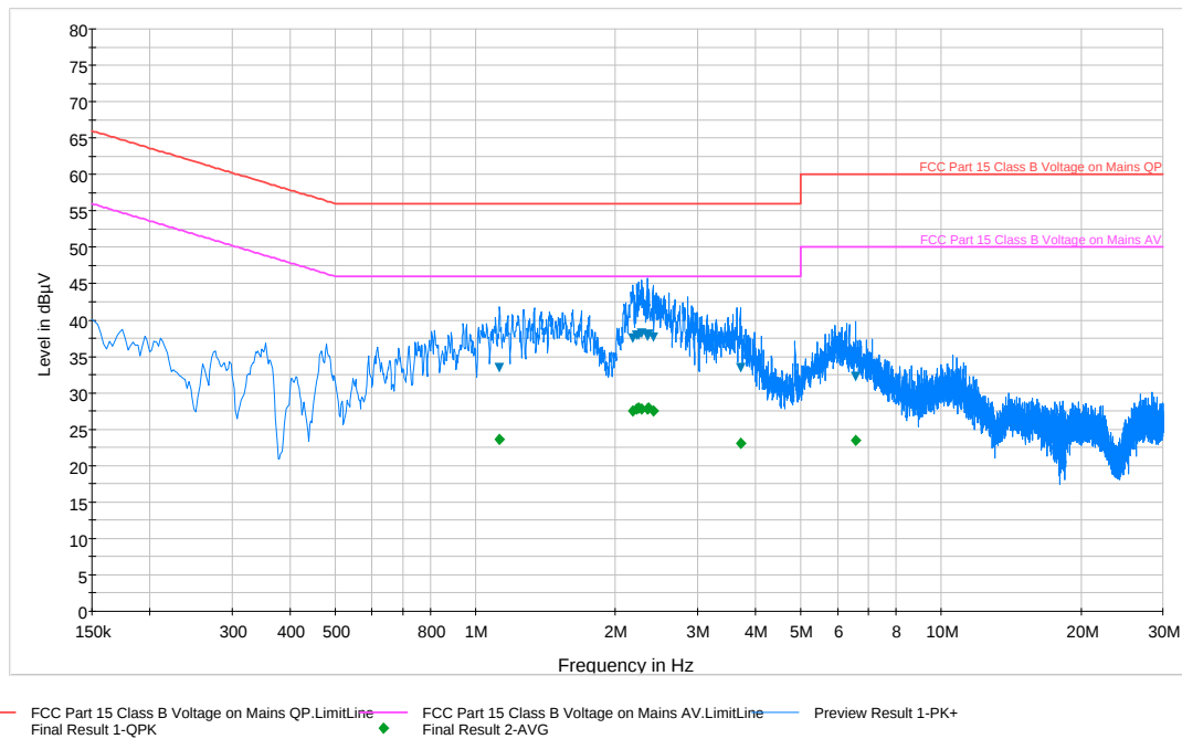
Plot 6-65. Line Conducted Data with 802.11a (LN)
