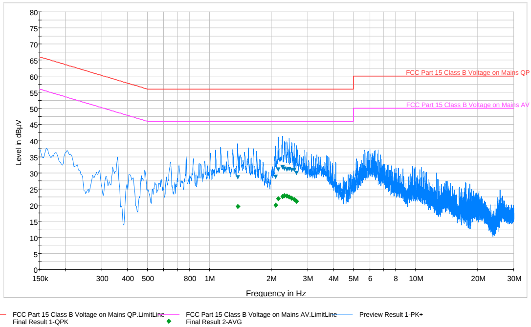
Plot 6-77. Line Conducted Plot with 802.11a (UNII Band 1) (L1)
