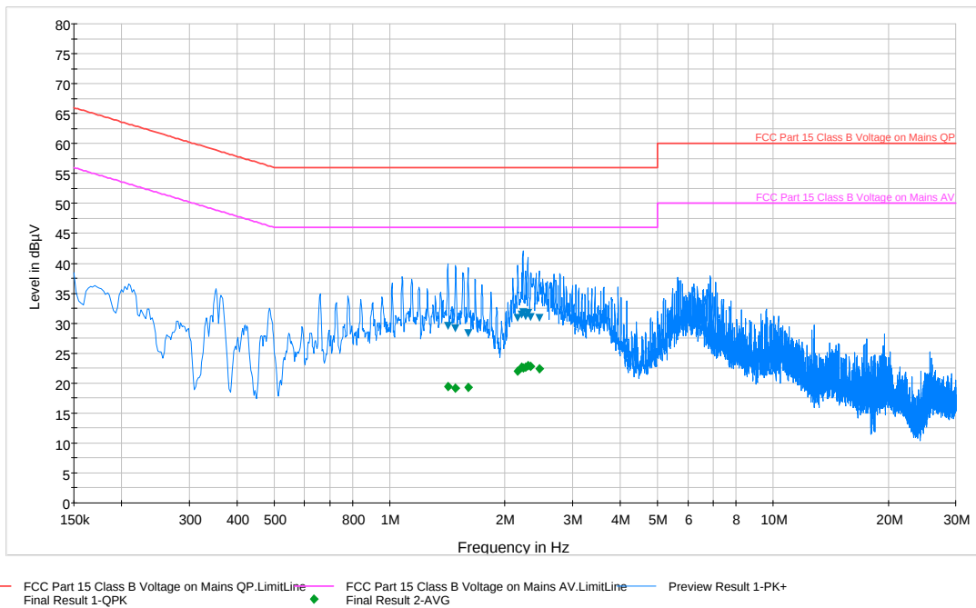
Plot 6-79. Line Conducted Plot with 802.11a (UNII Band 2) (L1)
