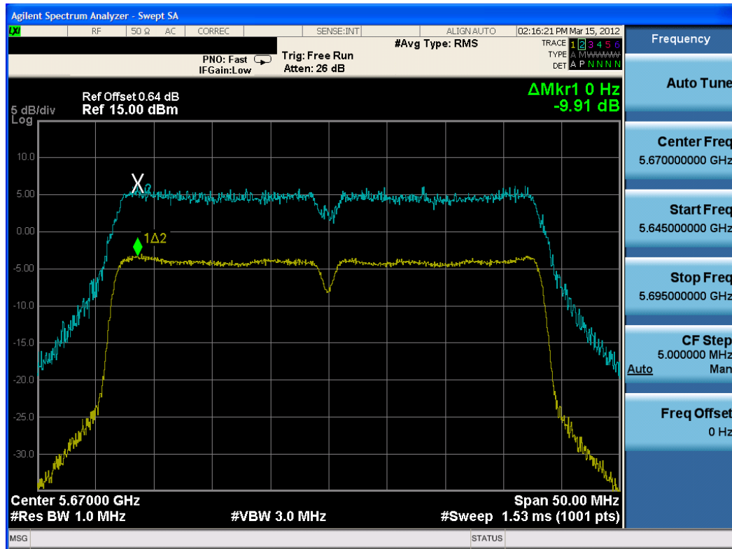
Plot 6-76. Peak Excursion Ratio Plot (802.11n – 40MHz BW (UNII Band 3) – Ch. 134)
