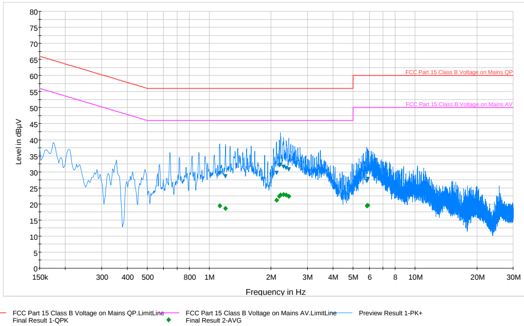
Plot 6-81. Line Conducted Plot with 802.11a (UNII Band 3) (L1)
