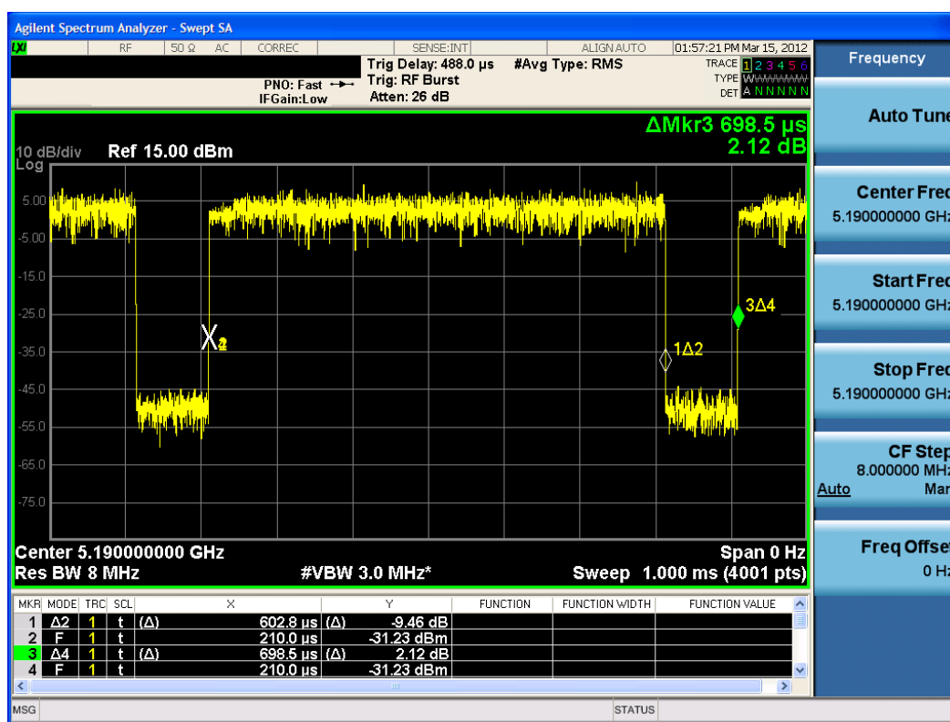
Plot 6-26. Pulse Width for 40MHz 802.11n Signal at MCS0 Data Rate
