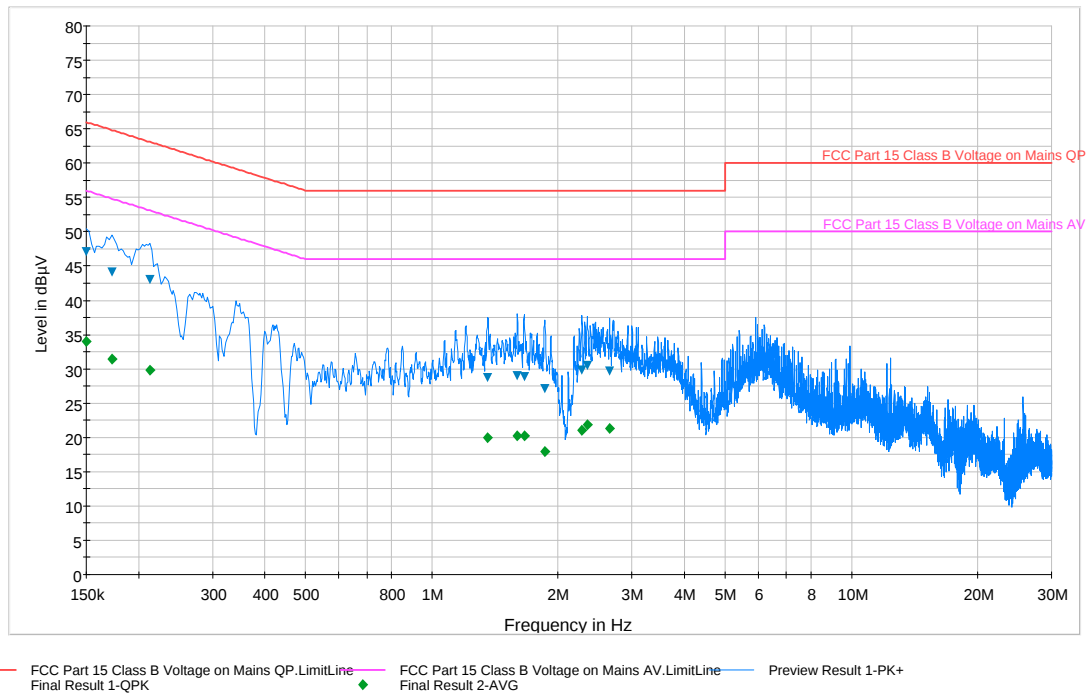
Plot 6-24. Line Conducted Plot with Bluetooth (L1)
