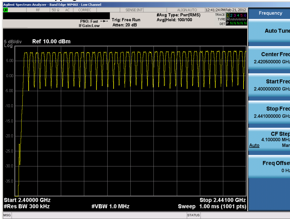
Plot 6-16. Low End Spectrum Channel Hopping Plot (Bluetooth)
