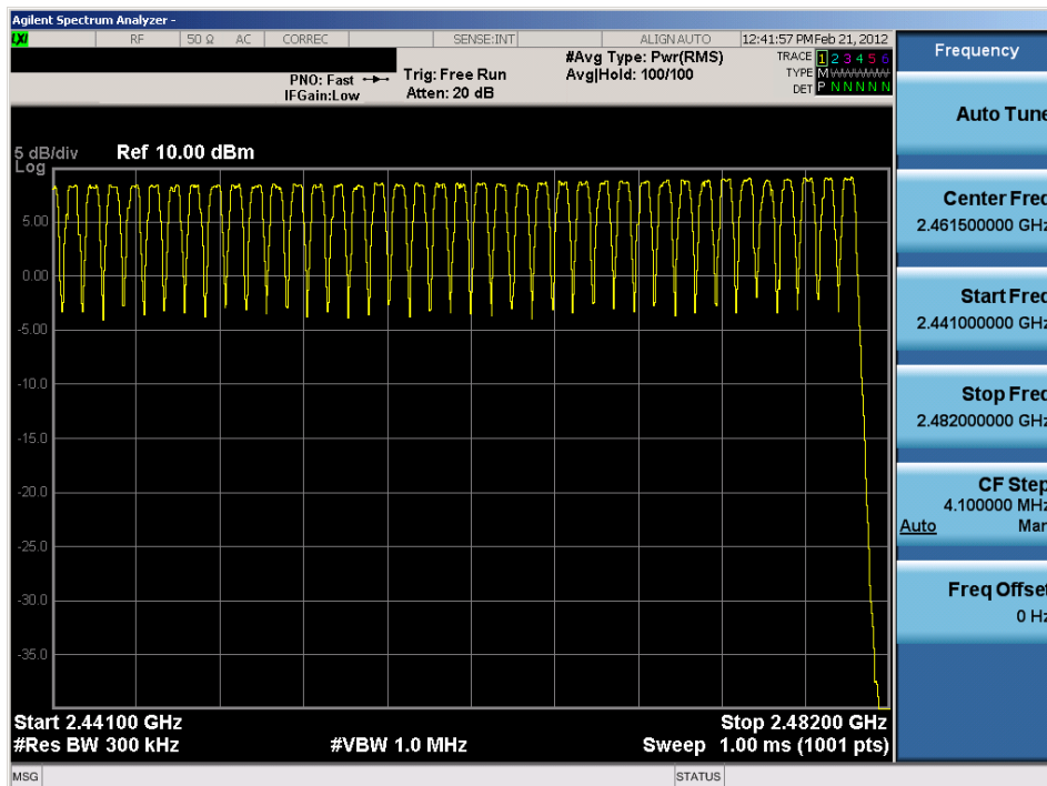
Plot 6-17. High End Spectrum Channel Hopping Plot (Bluetooth)
