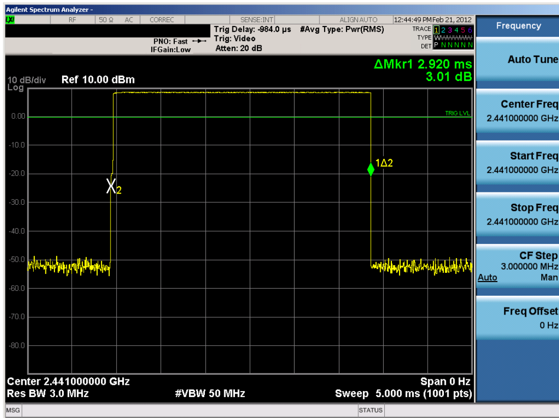
Plot 6-15. Time of Occupancy Plot (Bluetooth)
