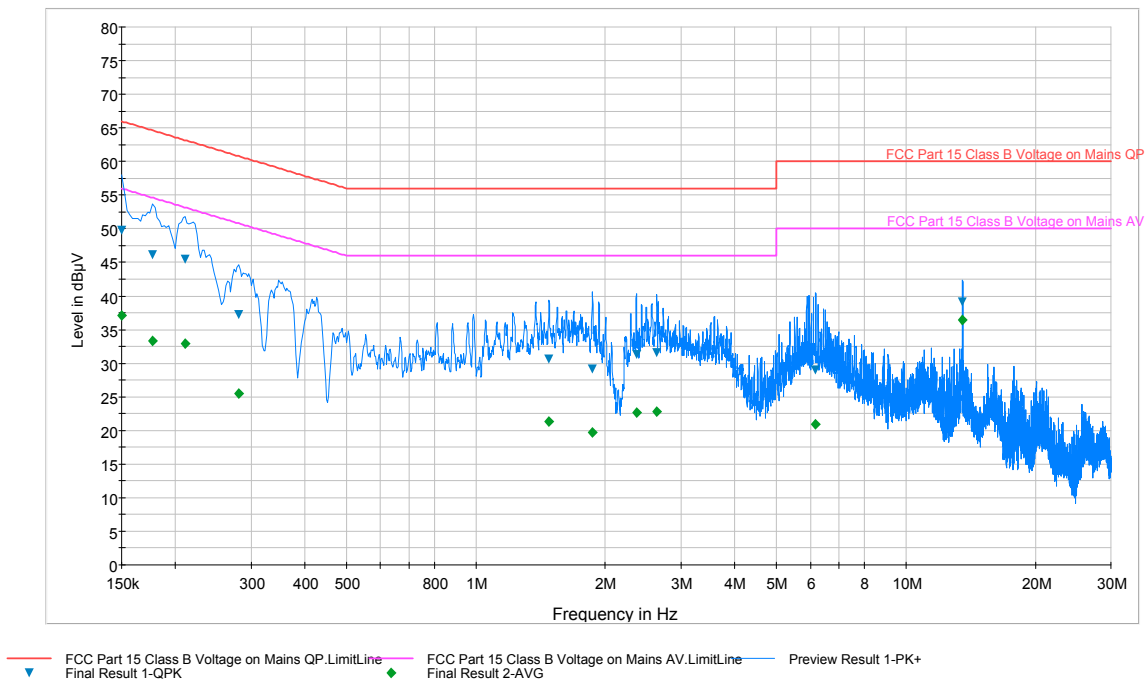
Plot 8-1. Line Conducted Plot (L1)
