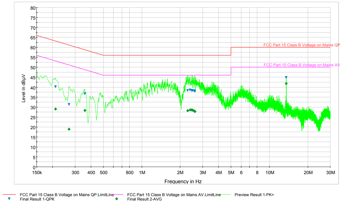
Plot 8-2. Line Conducted Plot (LN)
