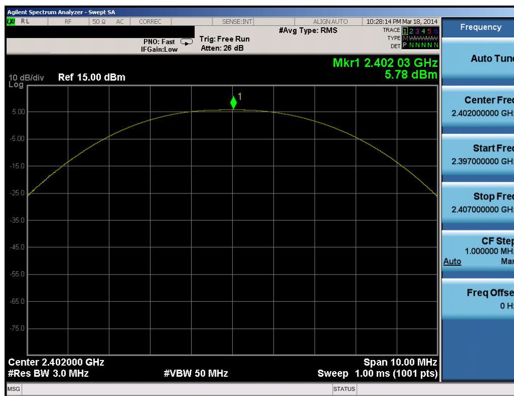
Plot 6-4. Peak Power Plot (Bluetooth (LE) – Ch. 0)
