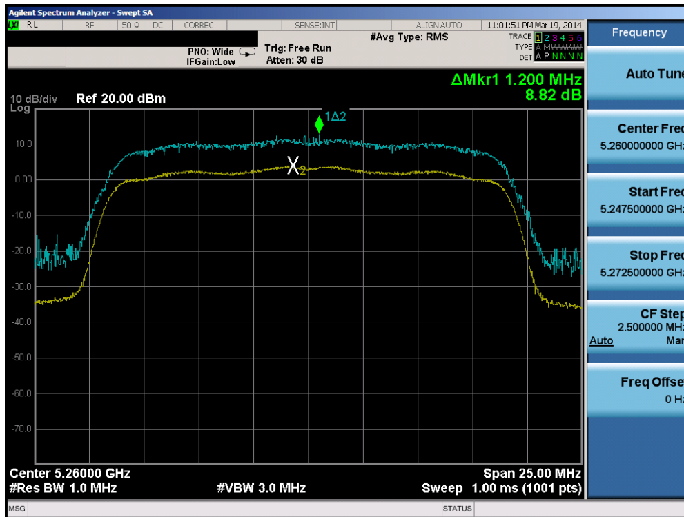
Plot 6-57. Peak Excursion Ratio Plot (20MHz BW 802.11n (UNII Band 2A) – Ch. 52)
