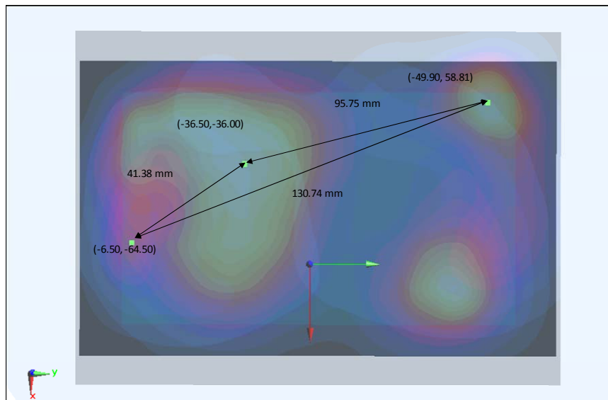
Figure 13-1 Peak SAR Location of 2.4 GHz WLAN and PCS CDMA at 10 mm
