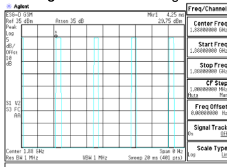
Figure 8-8 PCS GSM Signal
