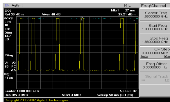
Figure 8-3 Zero-Span Plots
