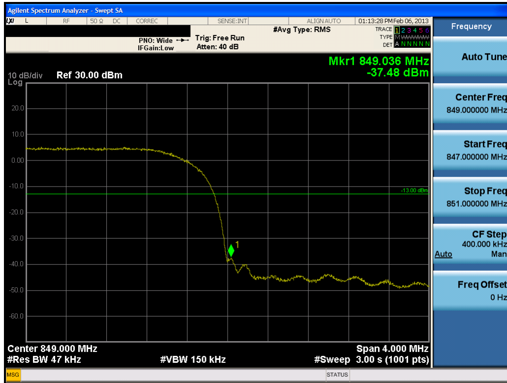
Plot 7-55. Band Edge Plot (Cellular WCDMA Mode – Ch. 4233)
