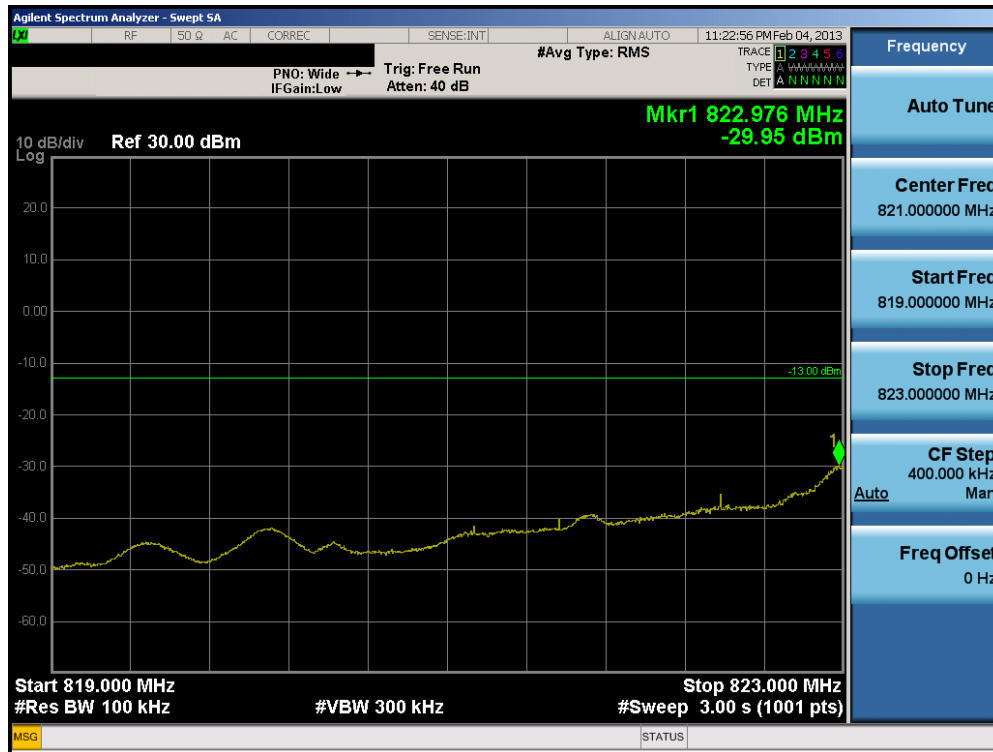
Plot 7-26. 4MHz Span Plot (Cellular CDMA Mode – Ch. 1013)
