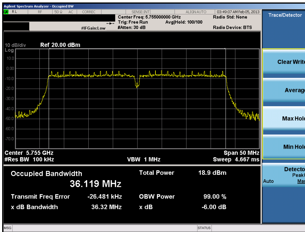
Plot 6-16. 6dB Bandwidth Plot (40MHz BW 802.11n (5.8GHz) – Ch. 151)
