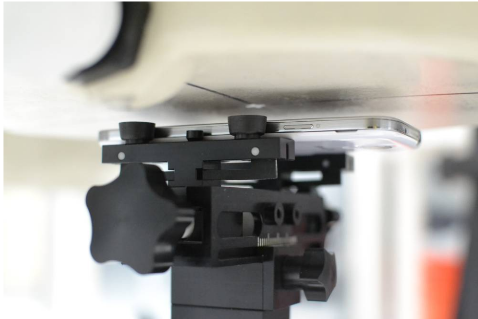
SAR Test Setup Photo 2 - Front Side at 1.0 cm
