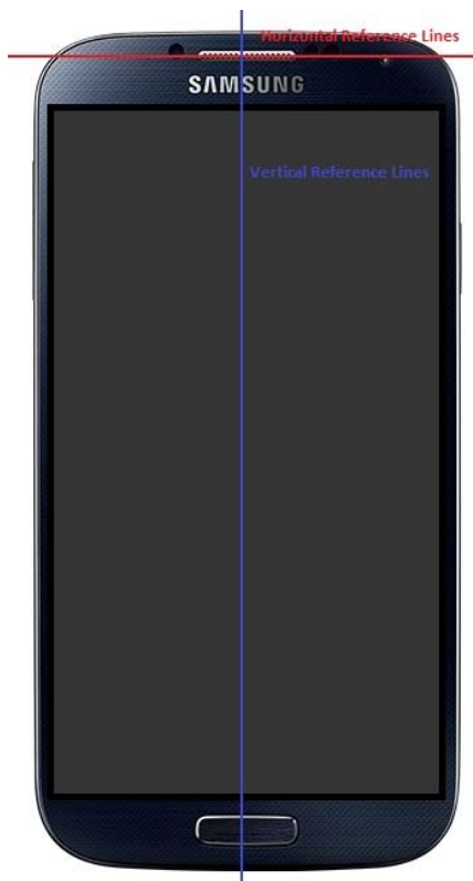
SAR Test Setup Photo 14 - Horizontal and Vertical Reference Lines
