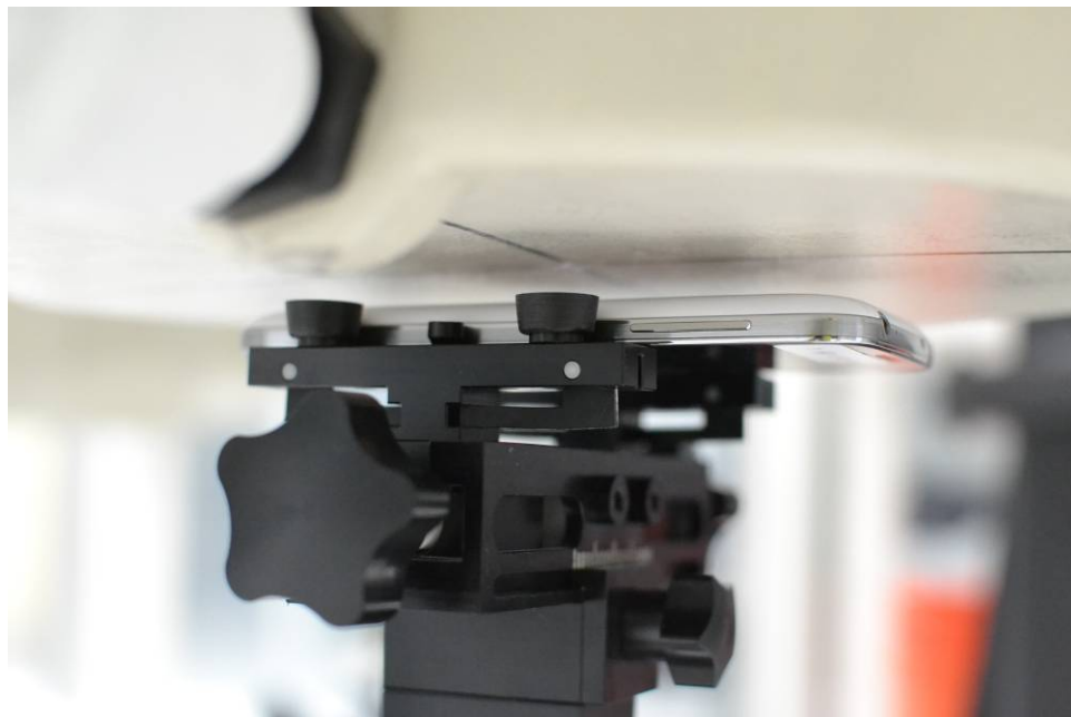
SAR Test Setup Photo 10 - Back Side with Wireless Charging Cover at 1.0 cm
