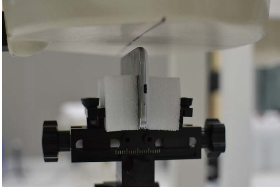
SAR Test Setup Photo 11 - Right Edge with Wireless Charging Cover at 1.0 cm
