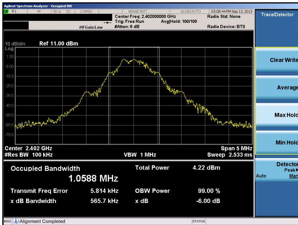
Plot 6-1. 6dB Bandwidth Plot (2402MHz – Low Channel)
