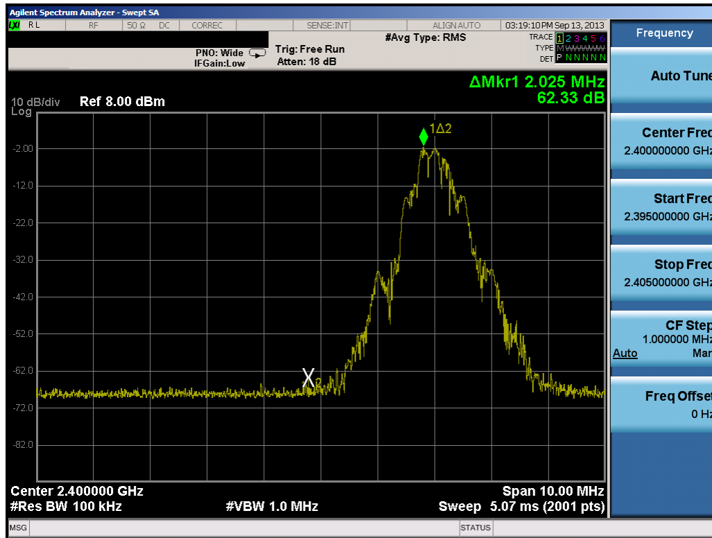
Plot 6-10. Band Edge Plot (Low Channel)
