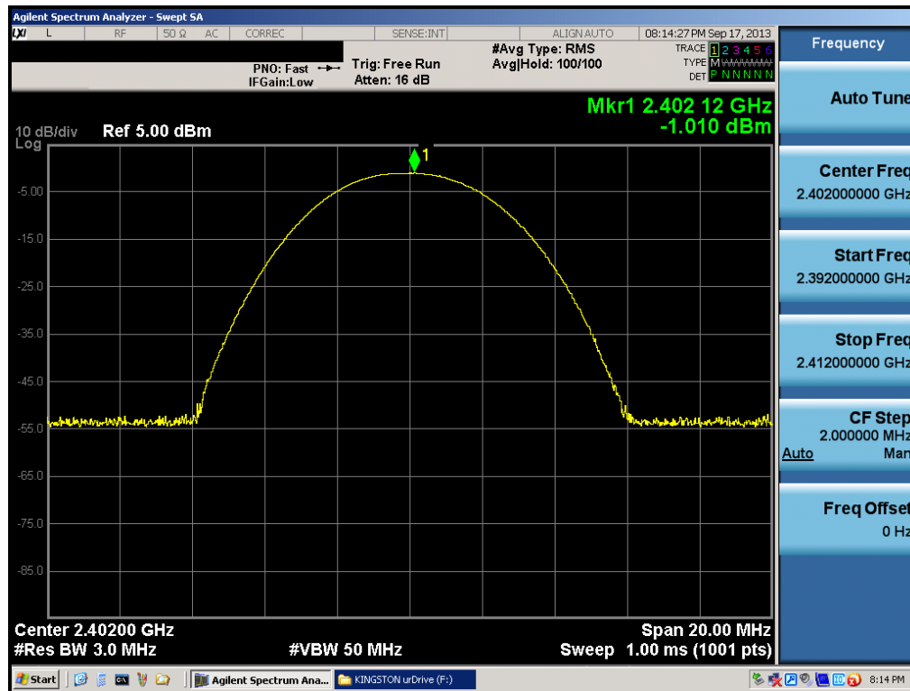
Plot 6-4. Peak Power Plot (2402MHz - Low Channel)
