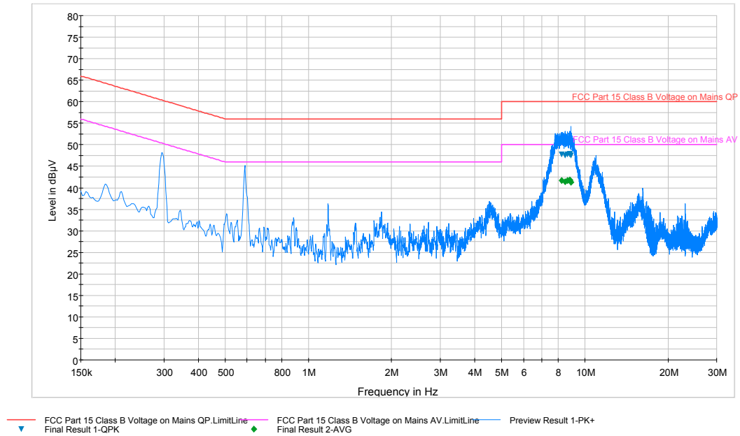
Plot 6-21. Line Conducted Plot with Ant+ (N)
