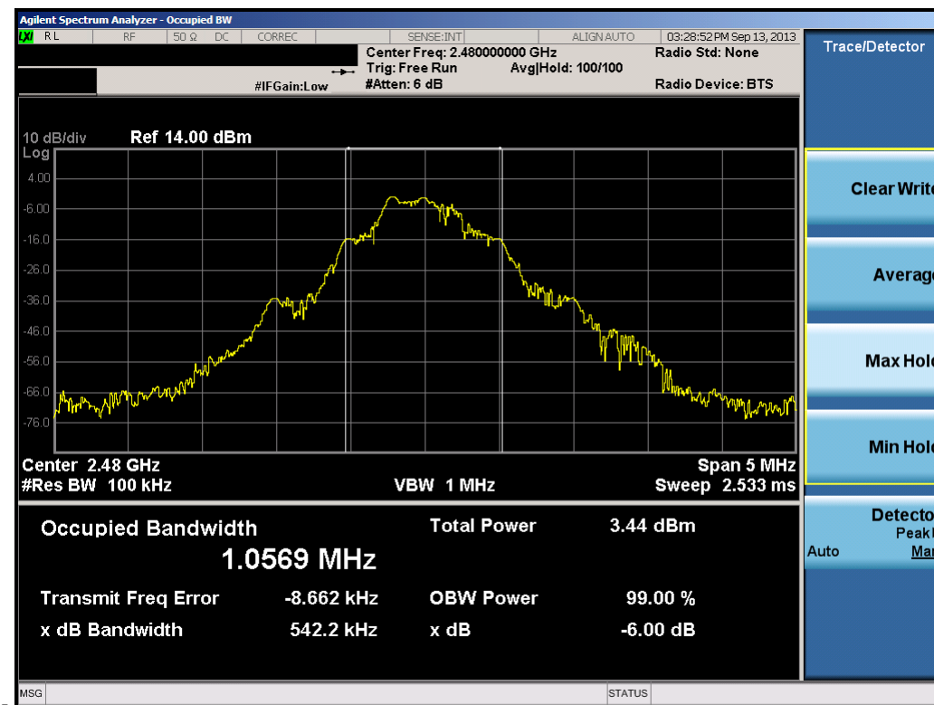
Plot 6-3. 6dB Bandwidth Plot (2480MHz – High Channel)
