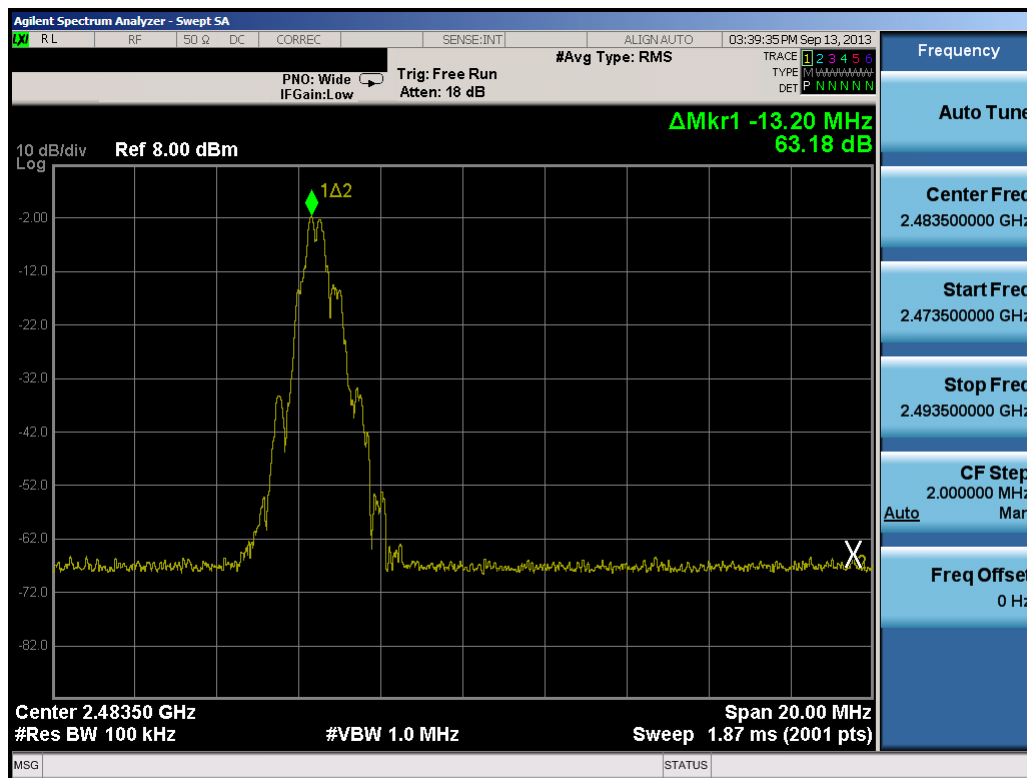
Plot 6-11. Band Edge Plot (High Channel)
