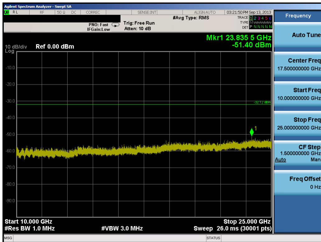
Plot 6-13. Conducted Spurious Plot (Low Channel)
