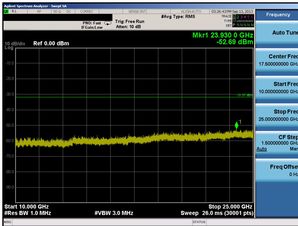
Plot 6-15. Conducted Spurious Plot (Mid Channel)
