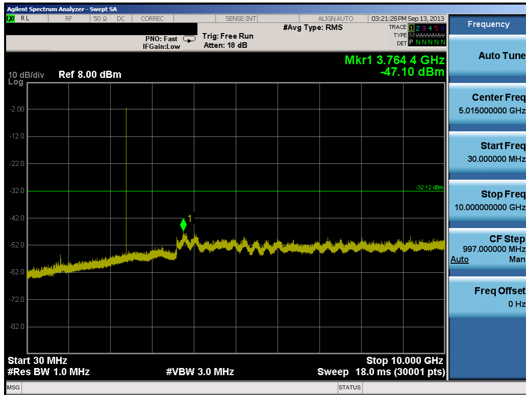
Plot 6-12. Conducted Spurious Plot (Low Channel)
