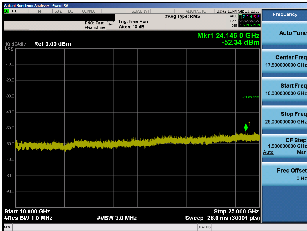
Plot 6-17. Conducted Spurious Plot (High Channel)
