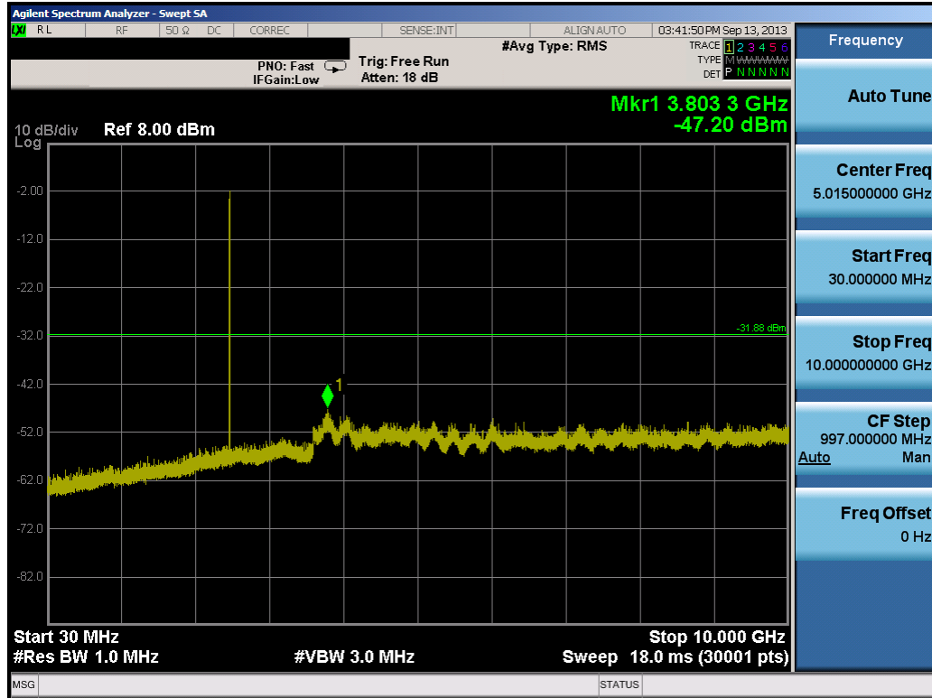
Plot 6-16. Conducted Spurious Plot (High Channel)
