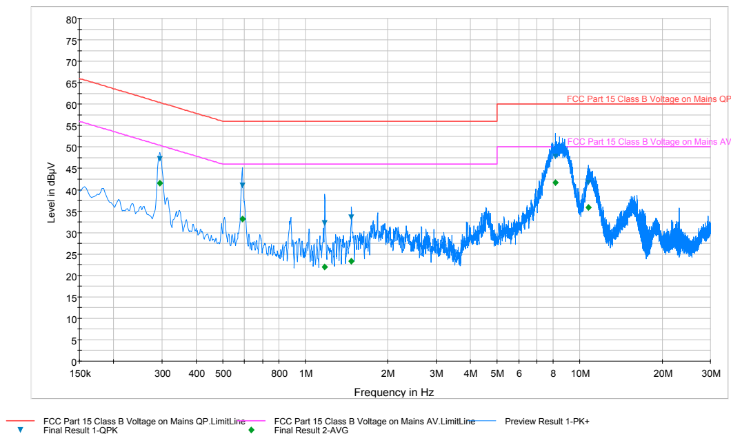
Plot 6-20. Line Conducted Plot with Ant+ (L1)
