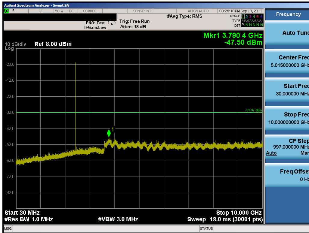
Plot 6-14. Conducted Spurious Plot (Mid Channel)
