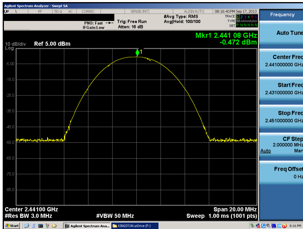
Plot 6-5. Peak Power Plot (2441MHz - Mid Channel)
