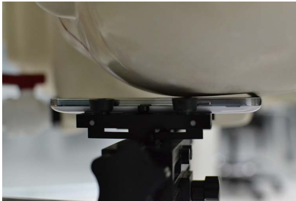
SAR Test Setup Photo 4 - Left Cheek, Wireless Charging Cover
