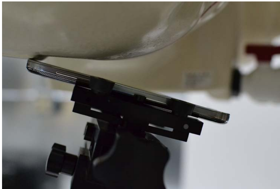
SAR Test Setup Photo 2 - Right Tilt, Standard Cover
