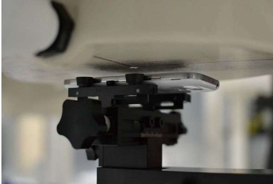
SAR Test Setup Photo 9 - Front Side at 1.0 cm, Wireless Charging Cover
