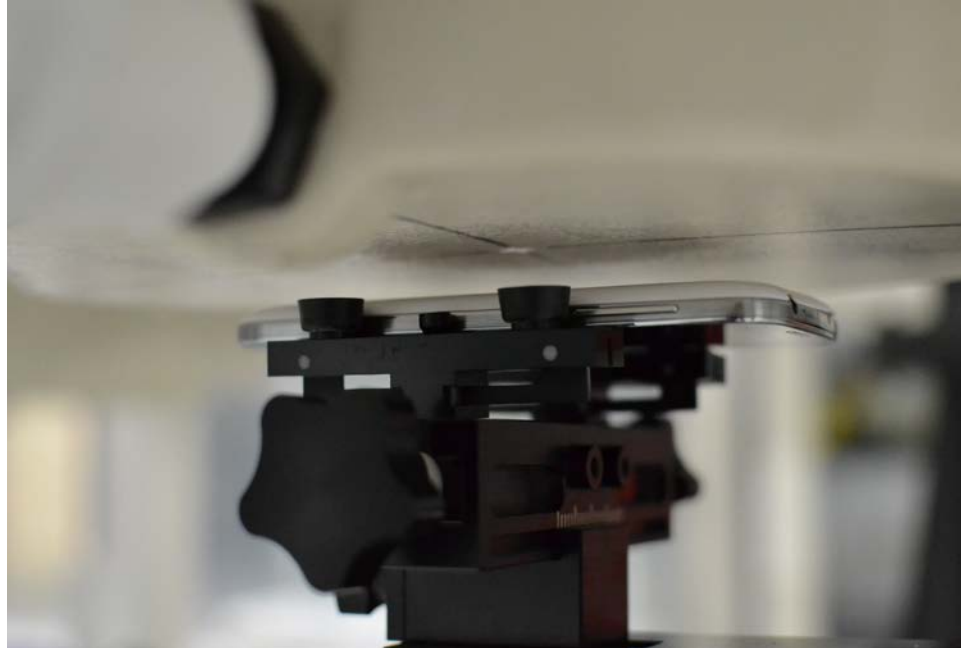
SAR Test Setup Photo 7 - Back Side at 1.0 cm, Wireless Charging Cover
