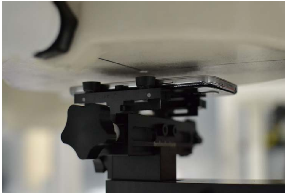
SAR Test Setup Photo 8 - Front Side at 1.0 cm, Standard Cover
