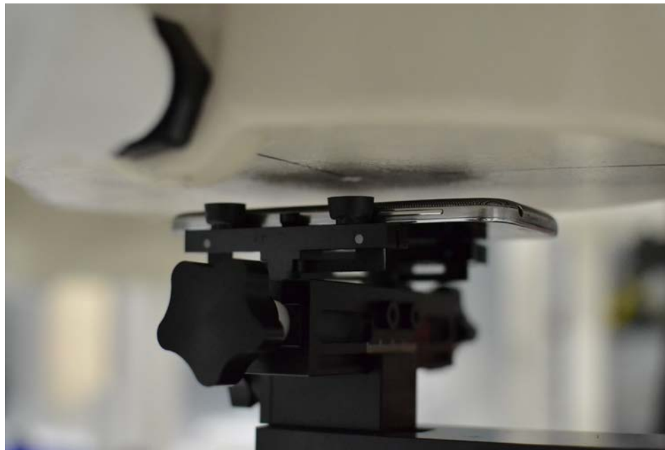
SAR Test Setup Photo 6 - Back Side at 1.0 cm, Standard Cover
