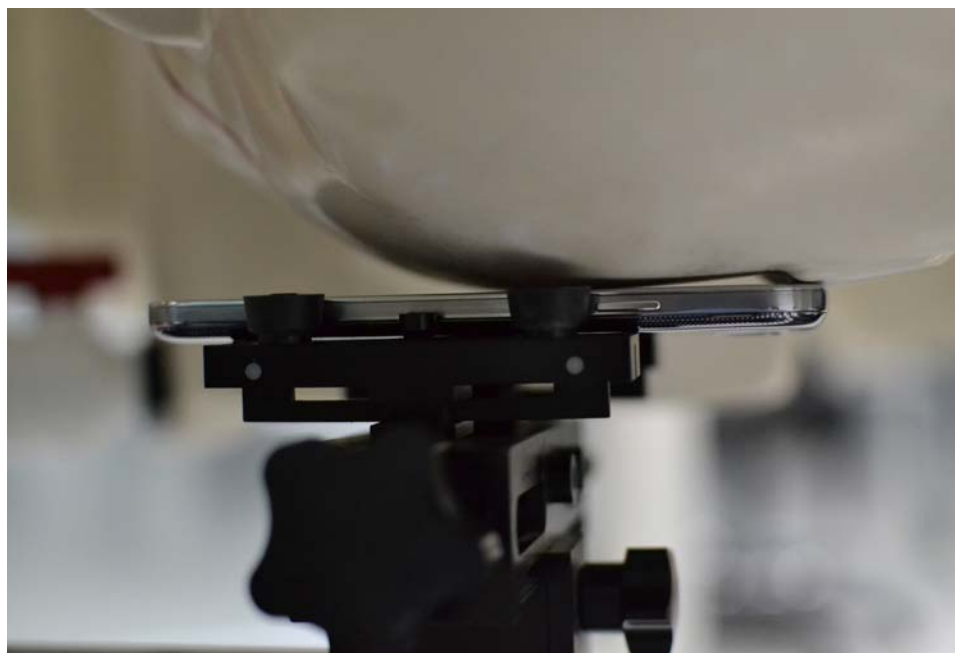
SAR Test Setup Photo 3 - Left Cheek, Standard Cover
