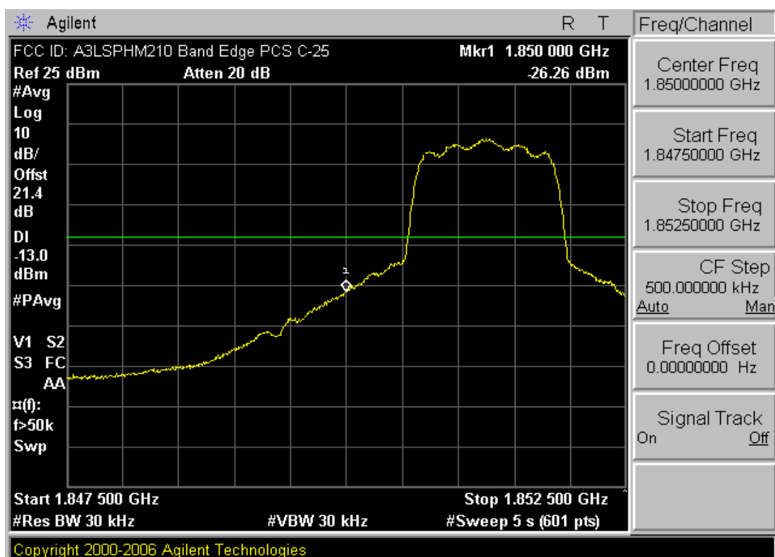
Plot 7-289. Band Edge Plot (PCS CDMA Mode – Ch. 25)
