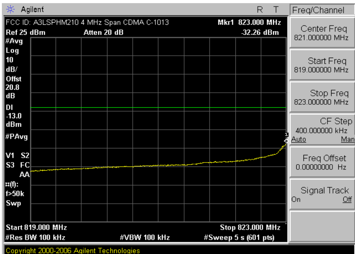
Plot 7-19. 4MHz Span Plot (Cellular CDMA Mode – Ch. 1013)
