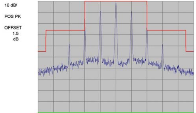
Plot 7-11. Signaling Tone (ST)
