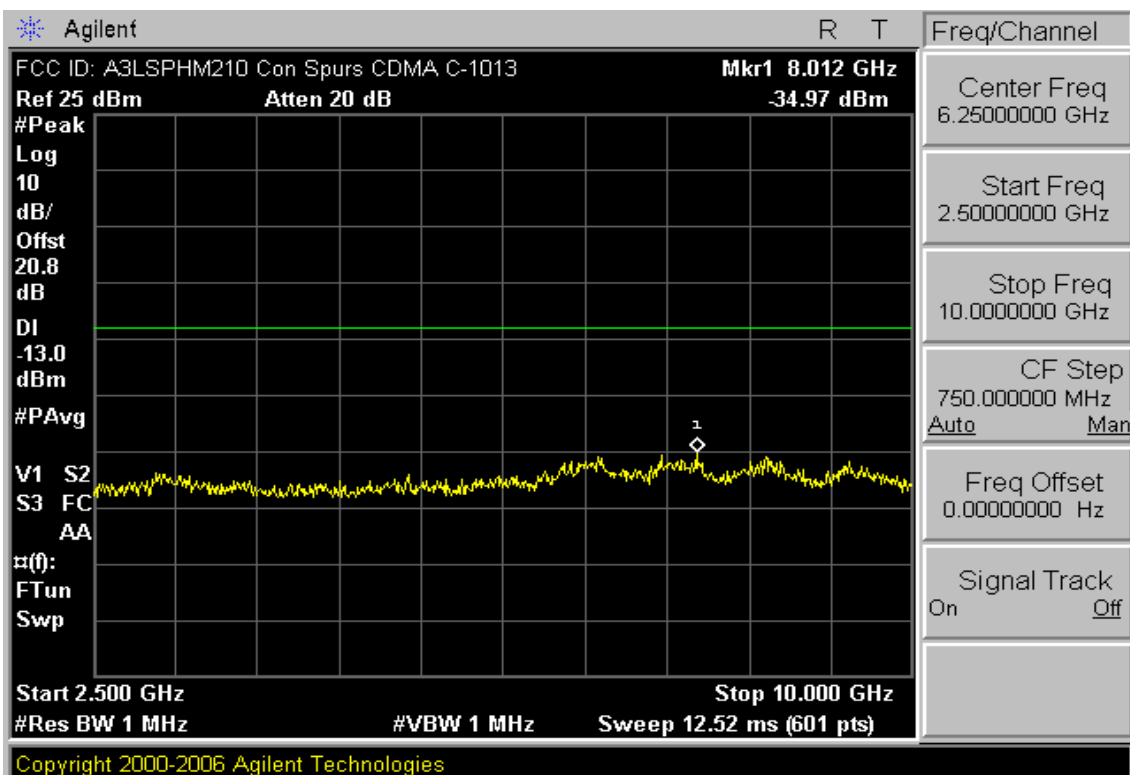
Plot 7-17. Conducted Spurious Plot (Cellular CDMA Mode – Ch. 1013)
