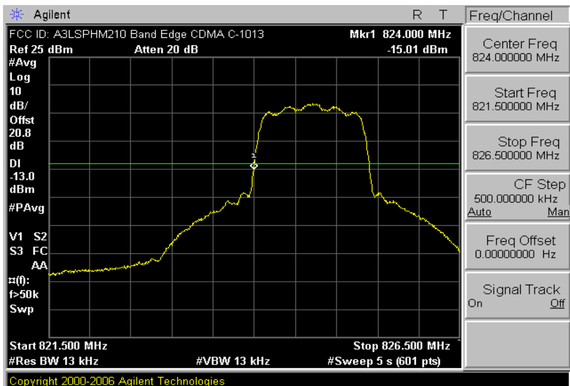
Plot 7-18. Band Edge Plot (Cellular CDMA Mode – Ch. 1013)
