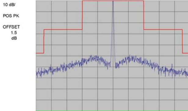
Plot 7-10. Unmodulated Signal
