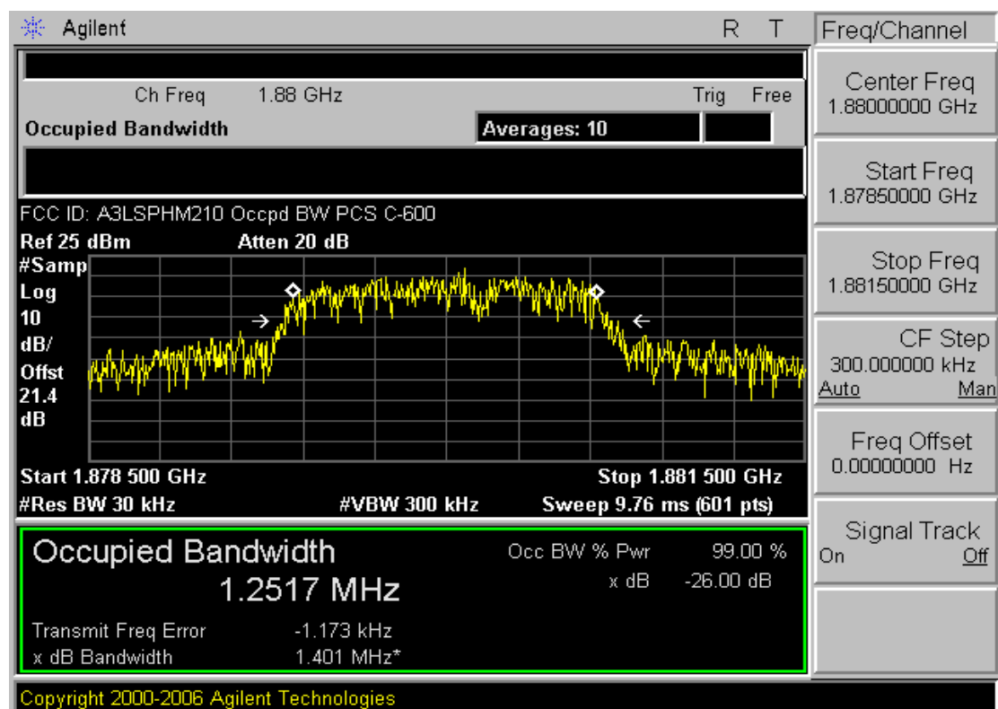
Plot 7-31. Occupied Bandwidth Plot (PCS CDMA Mode – Ch. 600)
