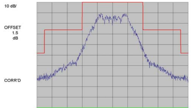
Plot 7-15. SAT + DTMF
