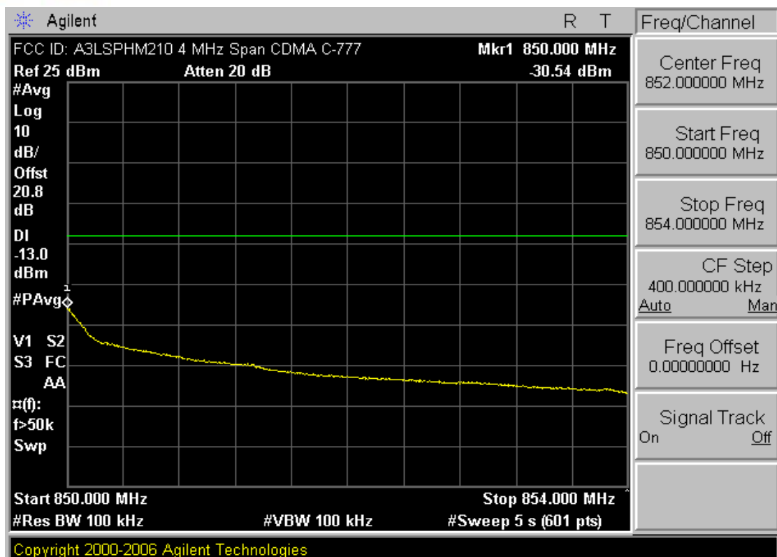
Plot 7-25. 4MHz Span Plot (Cellular CDMA Mode – Ch. 777)
