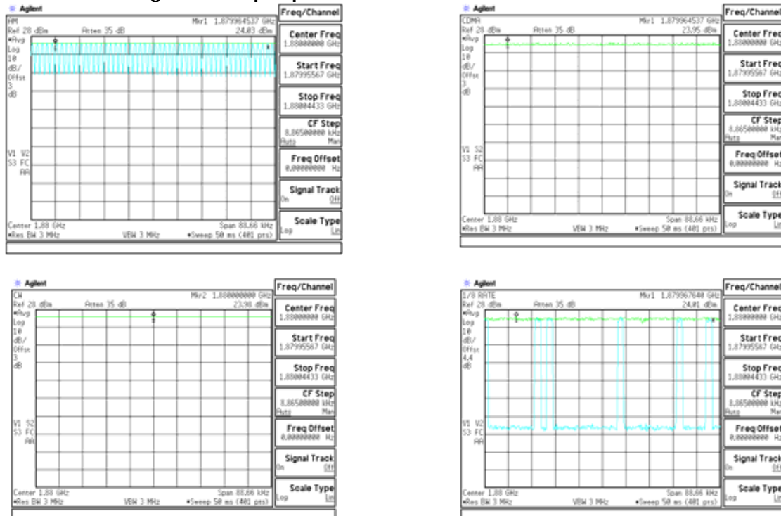
Figure 8-4 Zero-Span Plots
