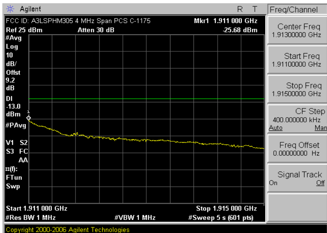
Plot 7-36. 4MHz Span Plot (PCS CDMA Mode – Ch. 1175)
