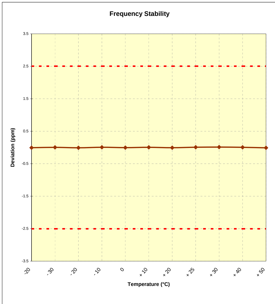
Figure 6-4. Frequency Stability Graph (PCS CDMA Mode – Ch. 600)
