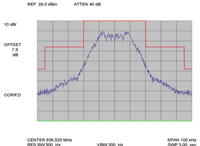
Plot 7-14. SAT + DTMF
