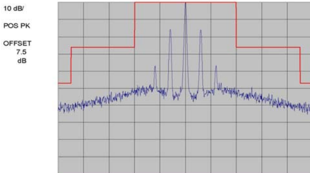
Plot 7-12. Supervisory Audio Tone (SAT)
