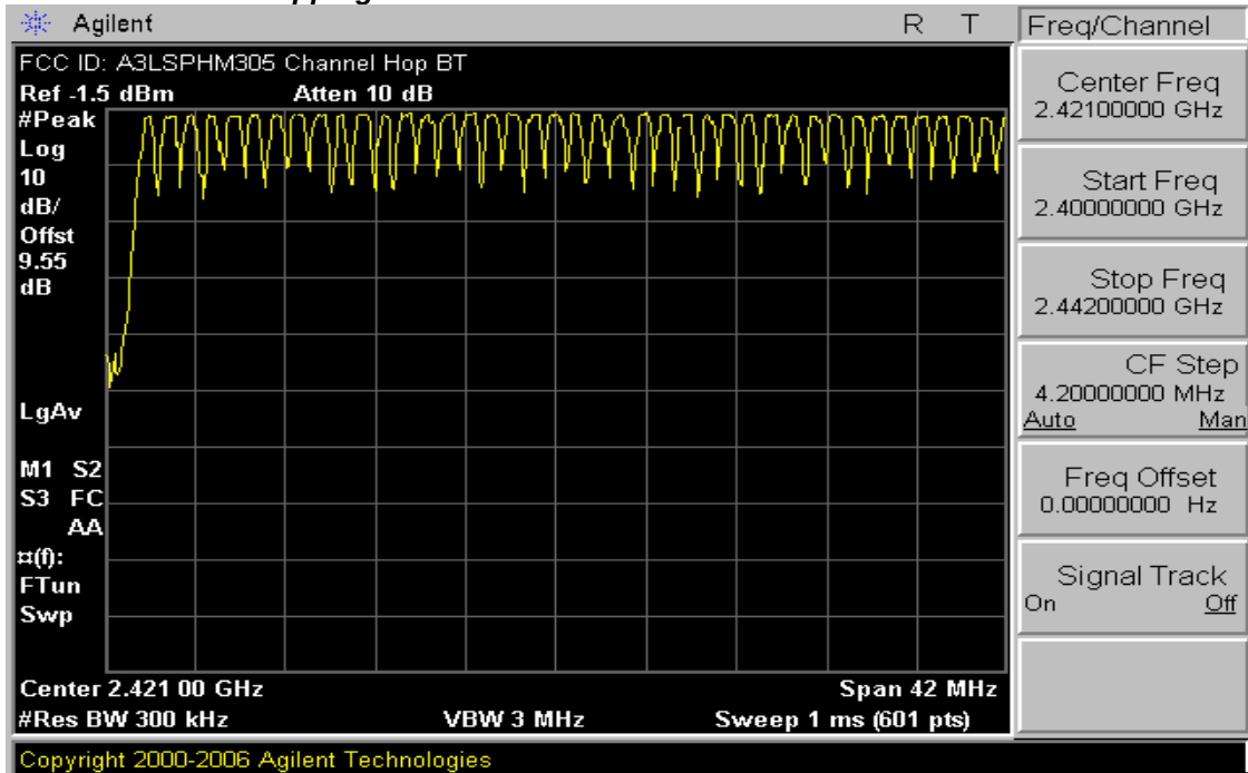
Plot 6-8. Low End Spectrum Channel Hopping Plot (Bluetooth)
