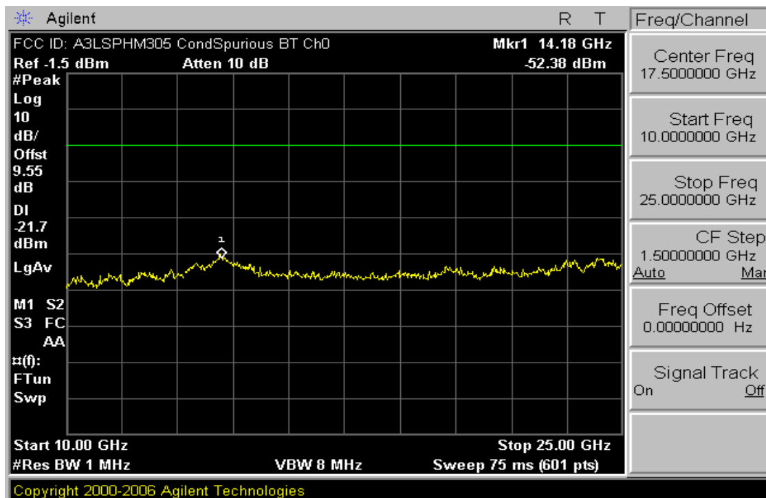
Plot 6-11. Conducted Spurious Plot (Bluetooth – Ch. 0)
