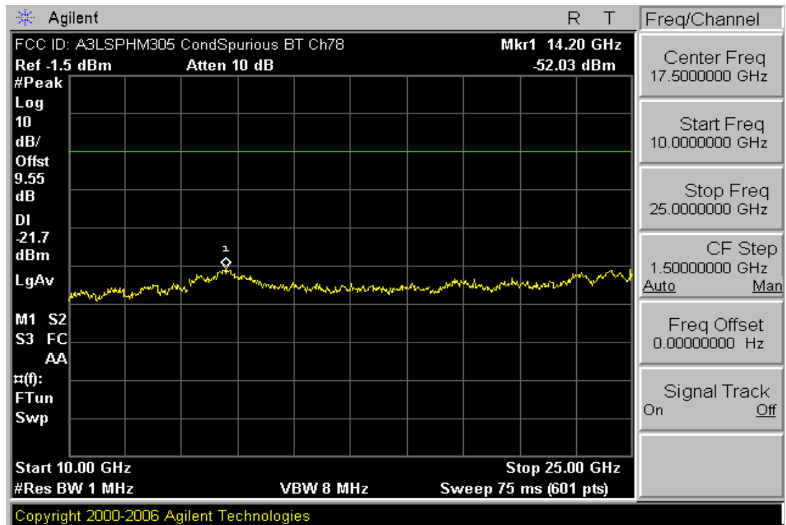
Plot 6-15. Conducted Spurious Plot (Bluetooth – Ch. 78)
