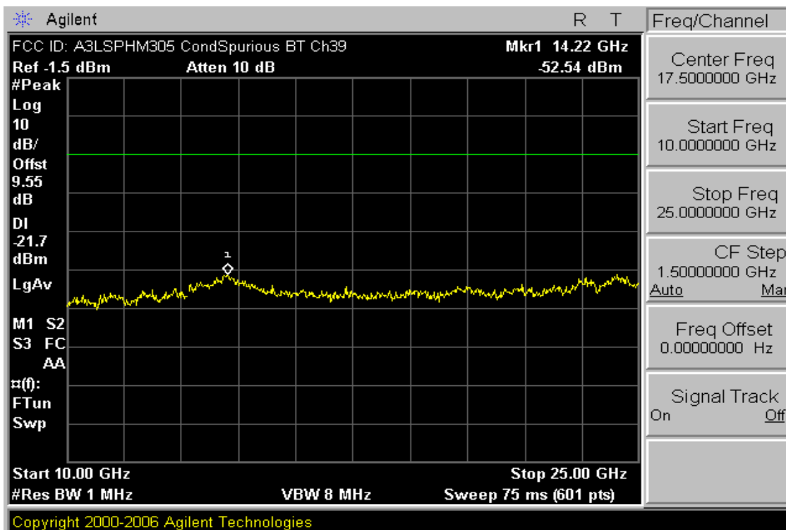
Plot 6-13. Conducted Spurious Plot (Bluetooth – Ch. 39)
