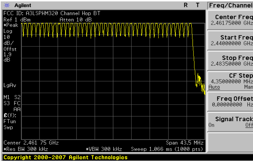
Plot 6-9. High End Spectrum Channel Hopping Plot (Bluetooth)
