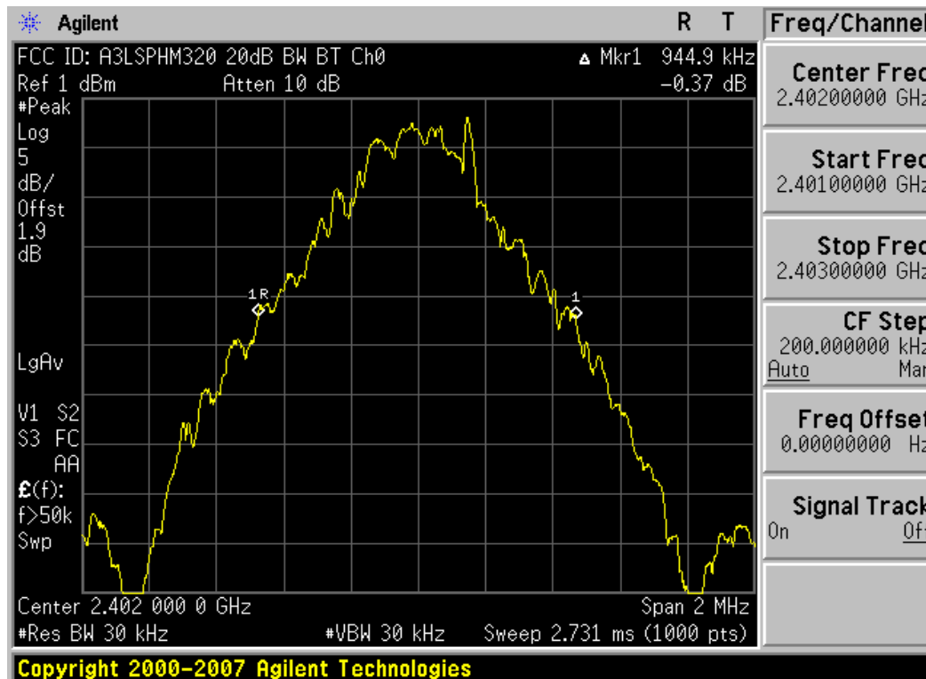
Plot 6-1. 20dB Bandwidth Plot (Bluetooth 2.0 – Ch. 0)
