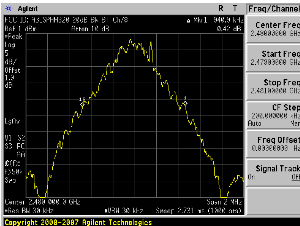
Plot 6-3. 20dB Bandwidth Plot (Bluetooth 2.0 – Ch. 78)
