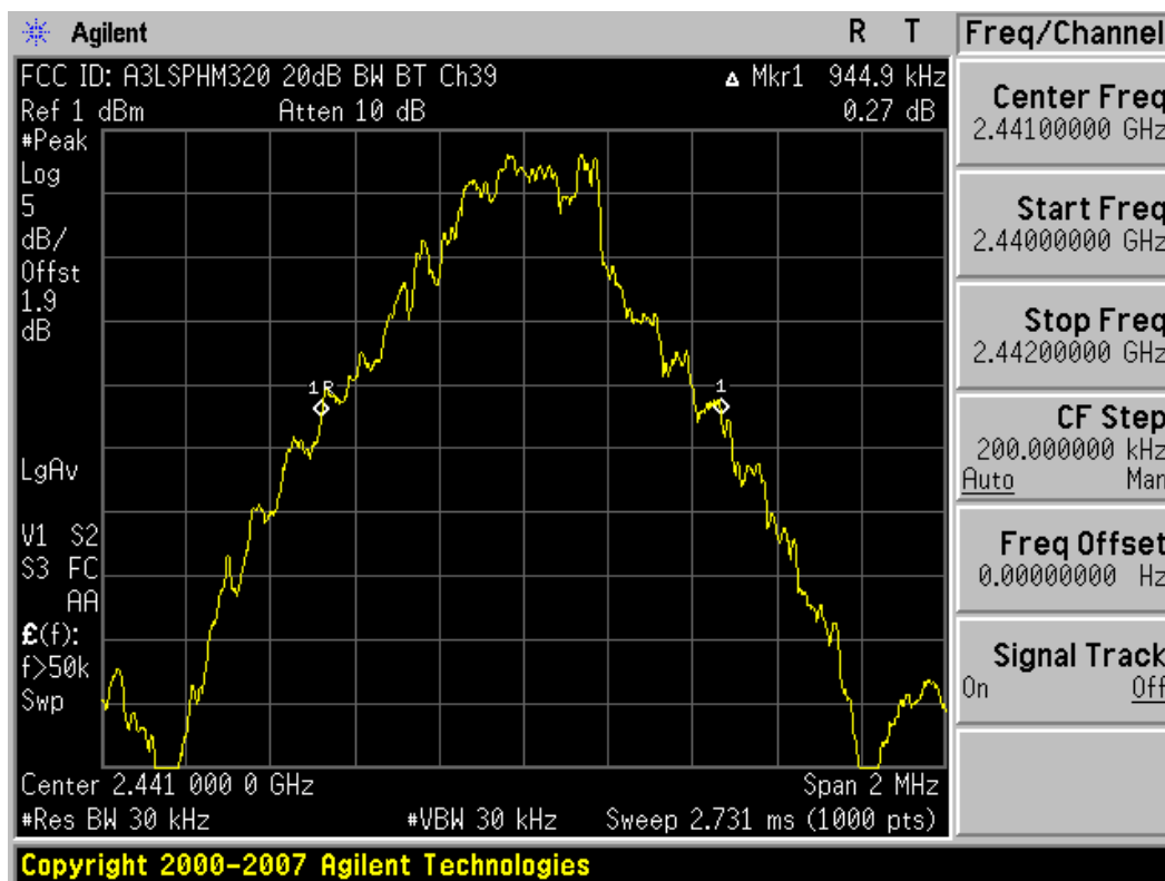
Plot 6-2. 20dB Bandwidth Plot (Bluetooth 2.0 – Ch. 39)
