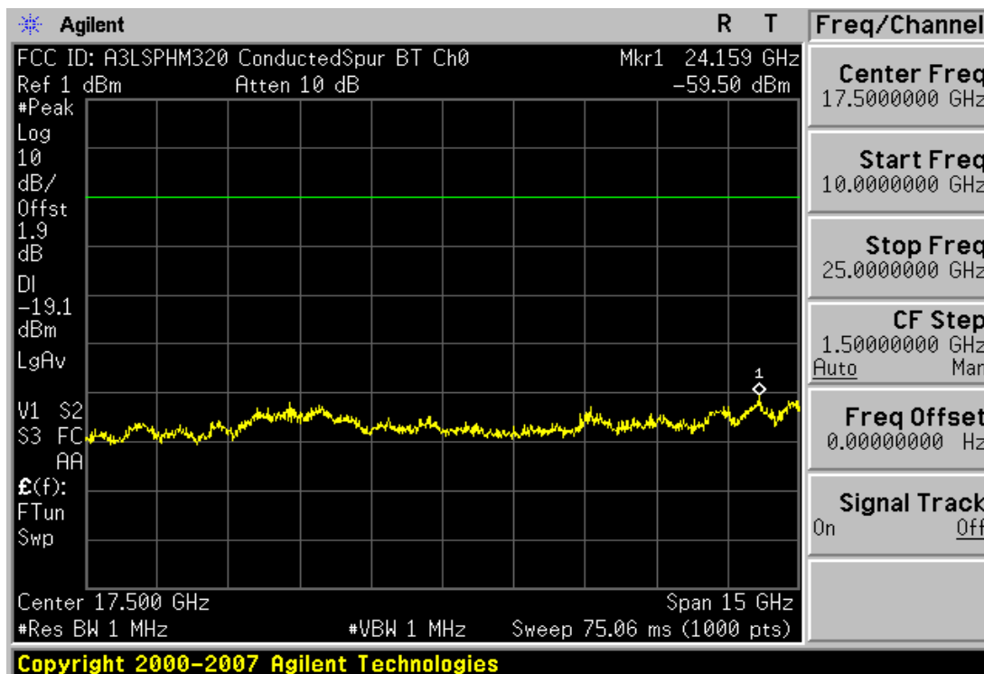
Plot 6-11. Conducted Spurious Plot (Bluetooth – Ch. 0)
