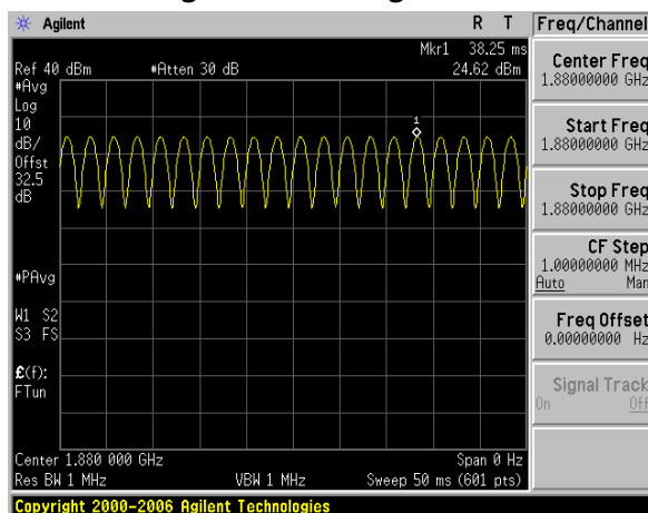
Figure 8.5 AM 80% Signal
