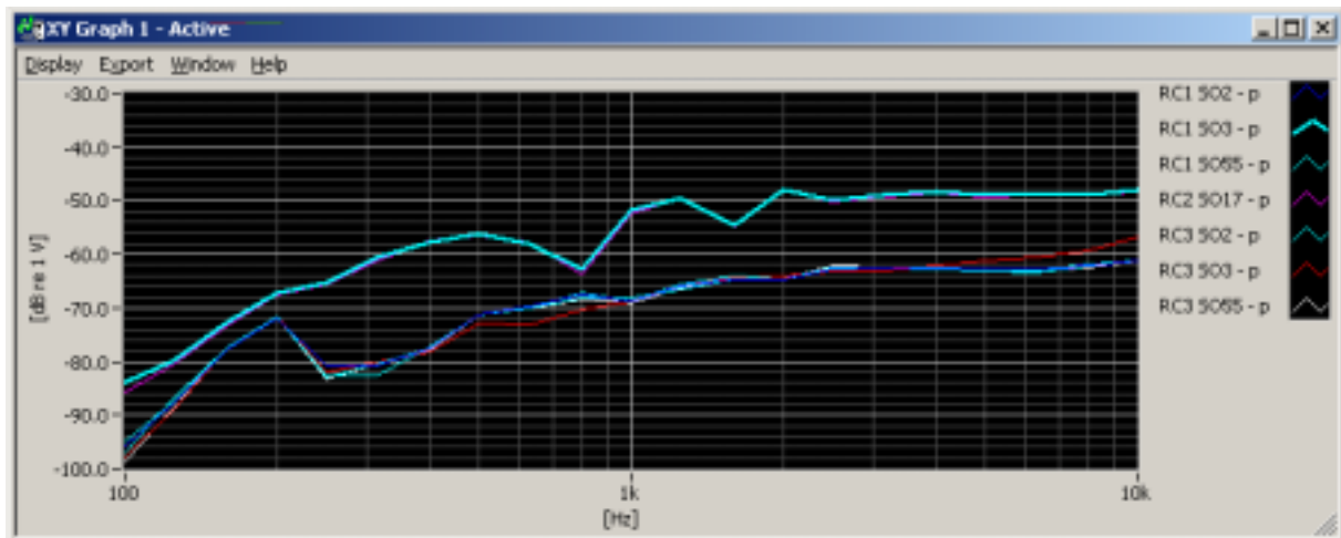
Figure 5-8 Vocoder Analysis for ABM Noise(CDMA)
