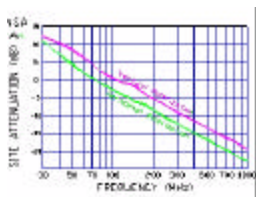
Figure 3-4. Normalized Site Attenuation Curves (H&V)
