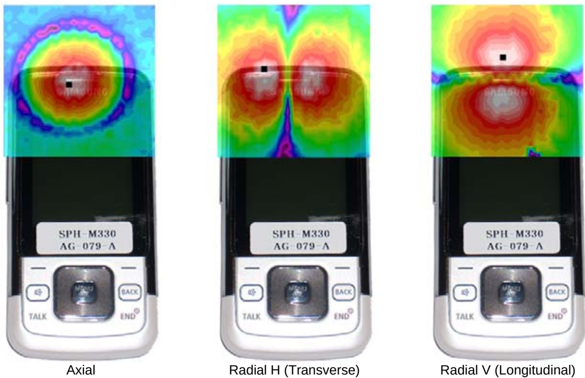
Figure 13-3 T-Coil Scan Overlay Magnetic Field Distributions
