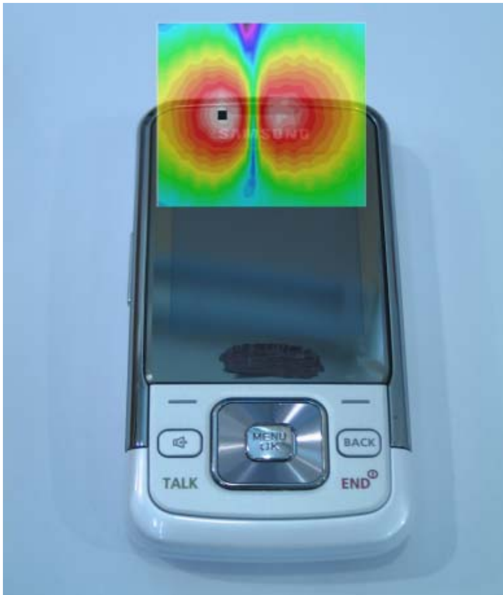
Slide Down Scan overlay with actual device (Radial Transverse)
