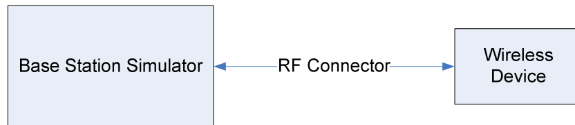
Figure 14-1 Power Measurement Setup
