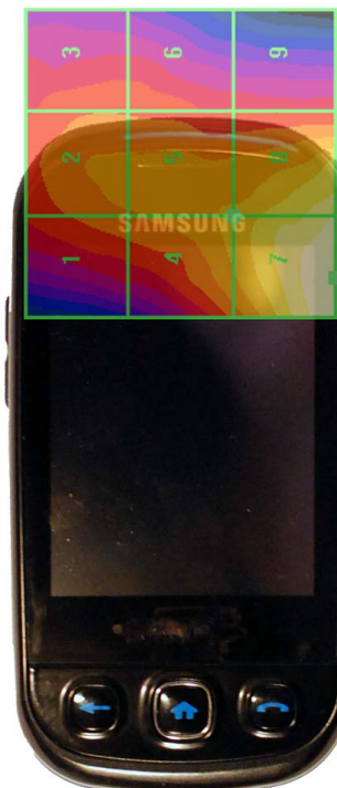
Figure 17-5 H-Field WD Scan overlay
