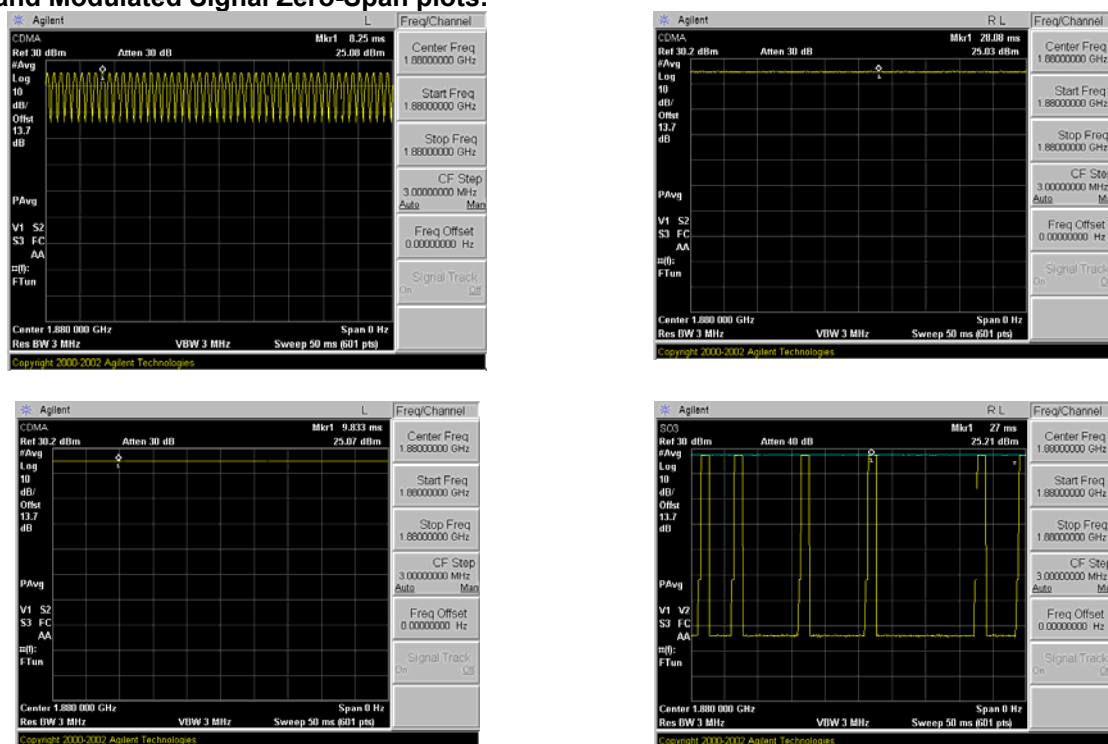
Figure 8-4 Zero-Span Plots
