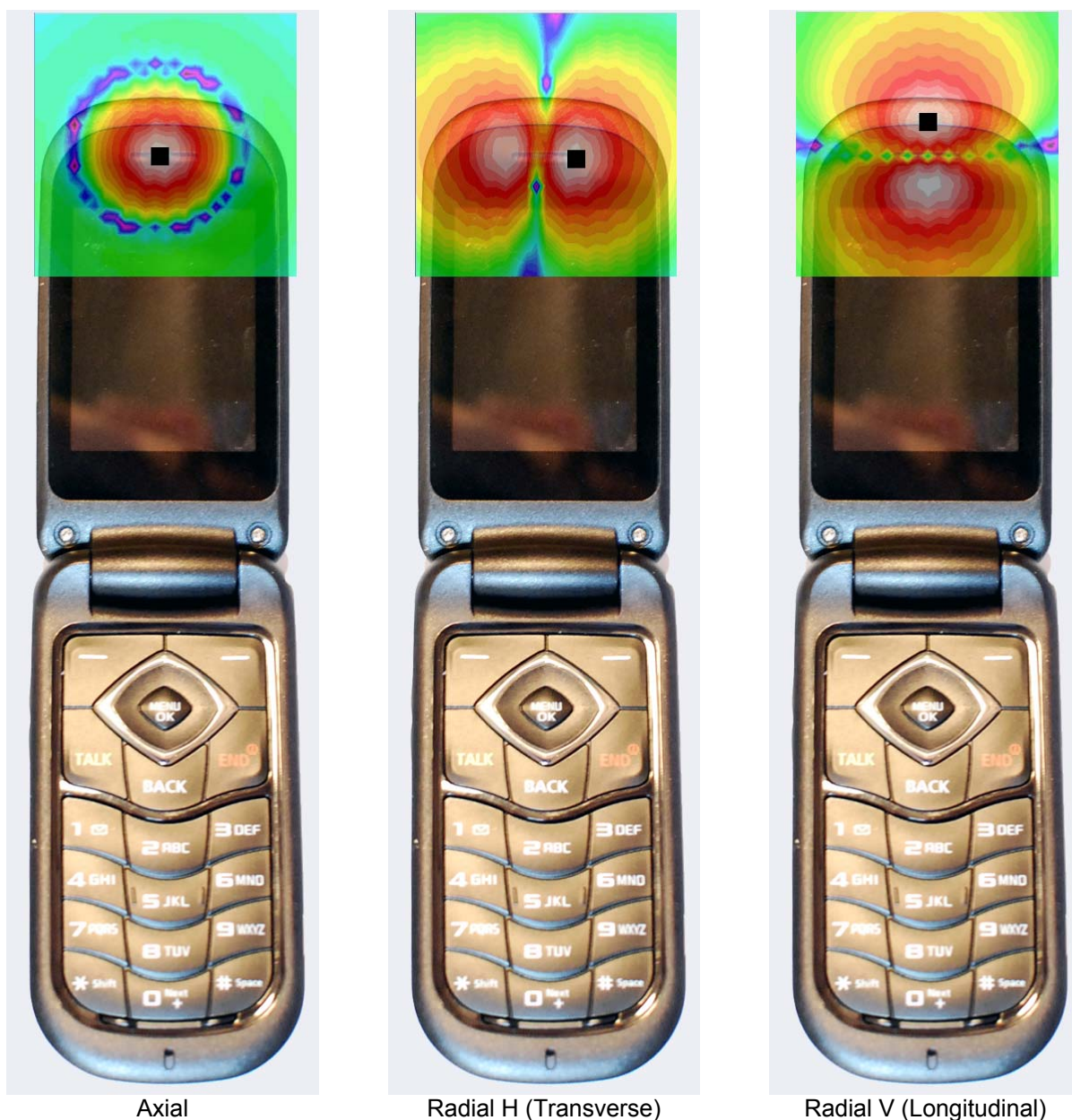
Figure 13-3 T-Coil Scan Overlay Magnetic Field Distributions
