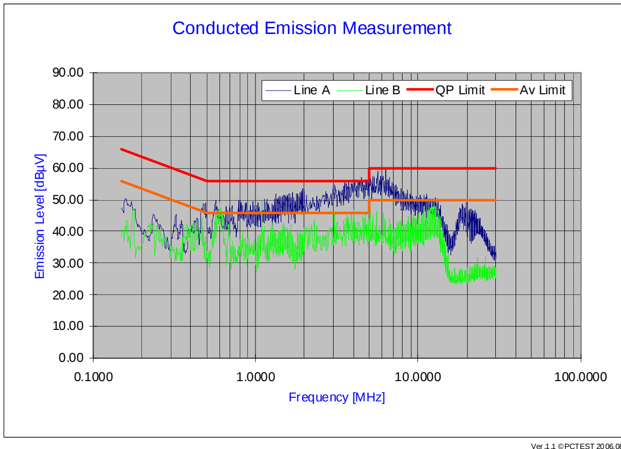
Plot 6-22. Line Conducted Plot with Bluetooth
