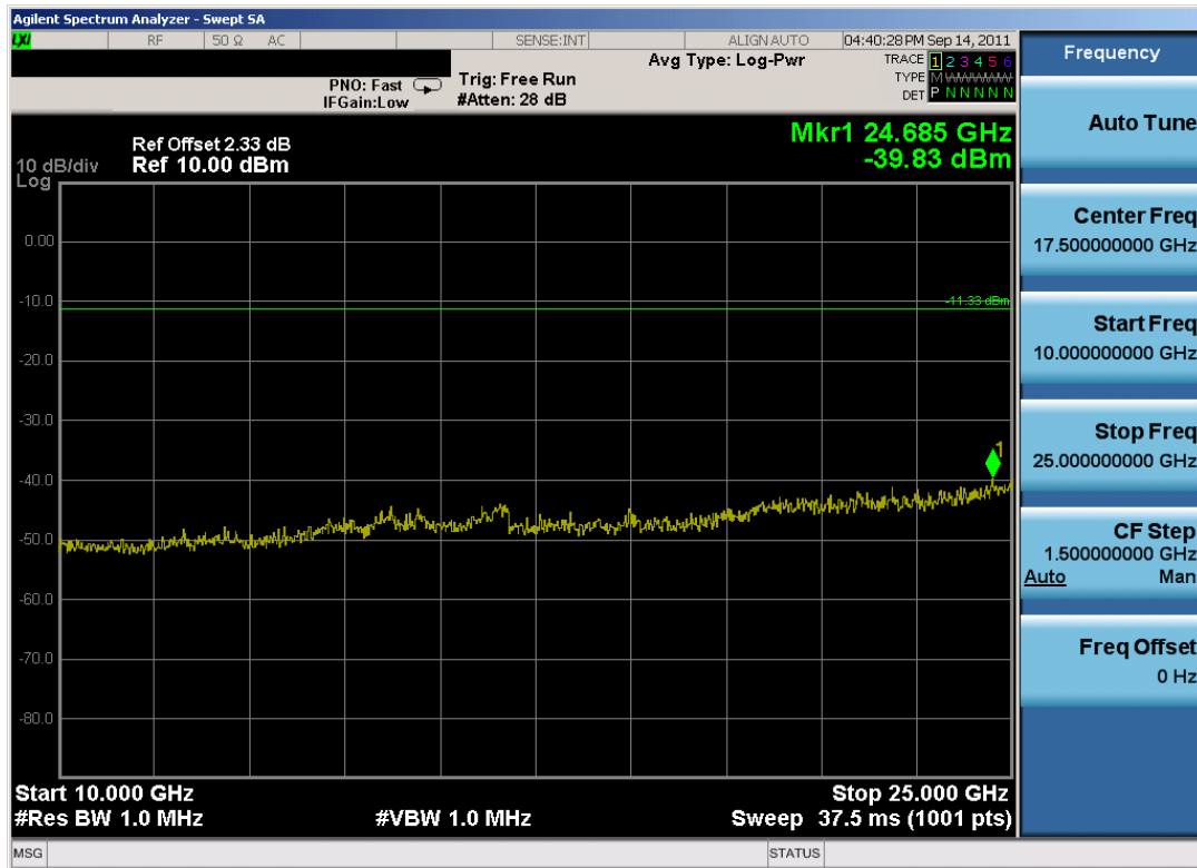
Plot 6-21. Conducted Spurious Plot (Bluetooth, 3Mbps – Ch. 78)
