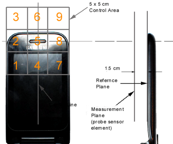
Figure 17-3 5x5 Scan grid above WD
