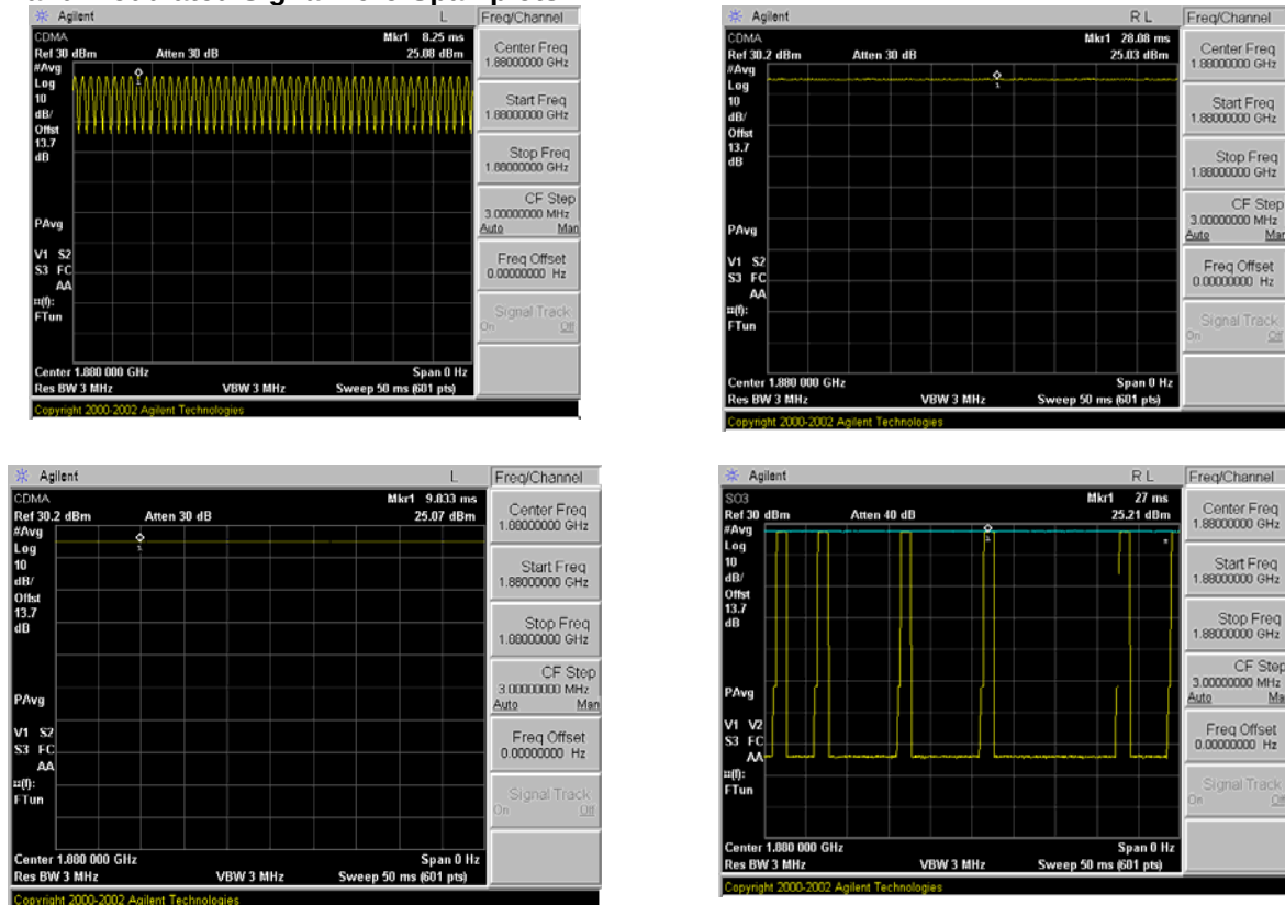
Figure 8-4 Zero-Span Plots
